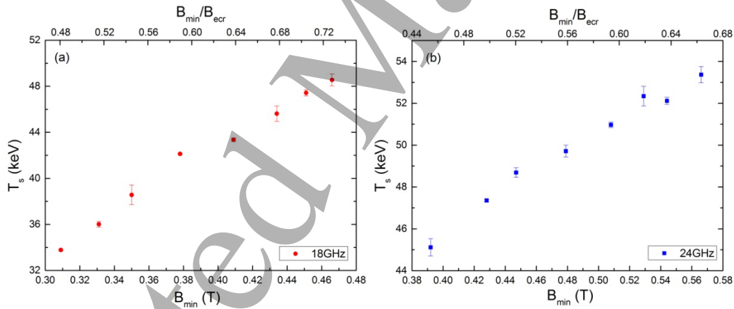
Figure 9: Spectral temperature T_s for 18 (a) and 24 (b) GHz heating at quasi-constant on-axis \nabla B_{eccr} .
