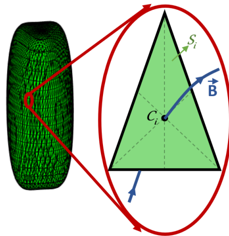
FIGURE 4.5 Three dimensional iso-magnetic field surface generation by dividing the surface into triangles and zoomed in view calculation of magnetic field gradient parallel to the magnetic field line \vec{B} through the centroid of the triangle C_i whose surface area is S_i .
