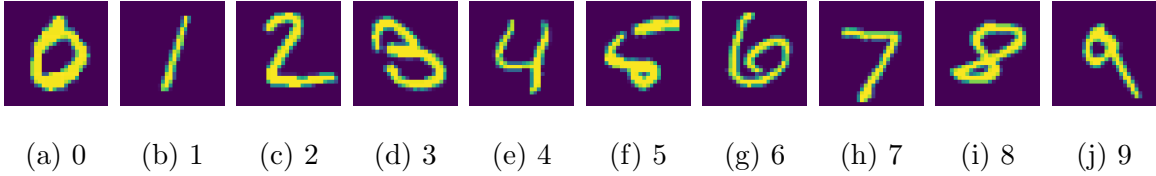
Figure 3.1: MNIST Images
