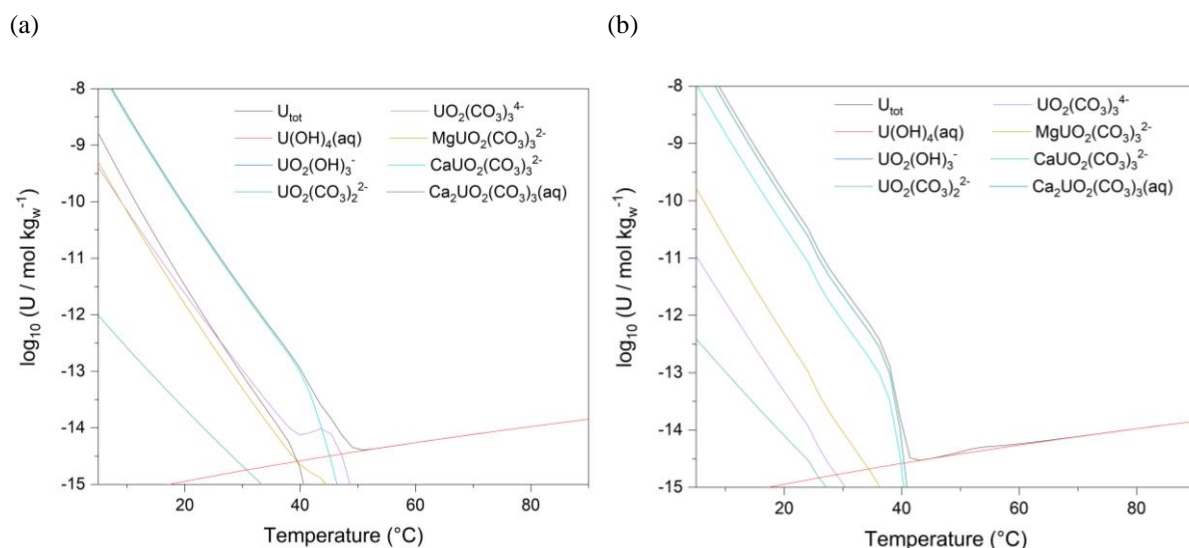
Fig. V - S7 Solubility of \text{UO}_2(\text{cr}) as a function of temperature (a) for Boom clay equilibrium waters, 11 P(\text{O}_2) = 10^{-68.67} atm and (b) for Callovo-Oxfordian clay equilibrium waters, 14 P(\text{O}_2) = 10^{-65.83} atm using thermodynamic data from the Thermochemie 10a database, 12 implementing \text{SrUO}_2(\text{CO}_3)_3^{2-} , 13 specific ion interaction coefficients of \text{Mg}_n/\text{Ca}_n\text{UO}_2(\text{CO}_3)_3^{(4-2n)-} 4-6 and their \Delta_r H_m^\circ values determined in this work based on the isoelectric reaction approximation.
