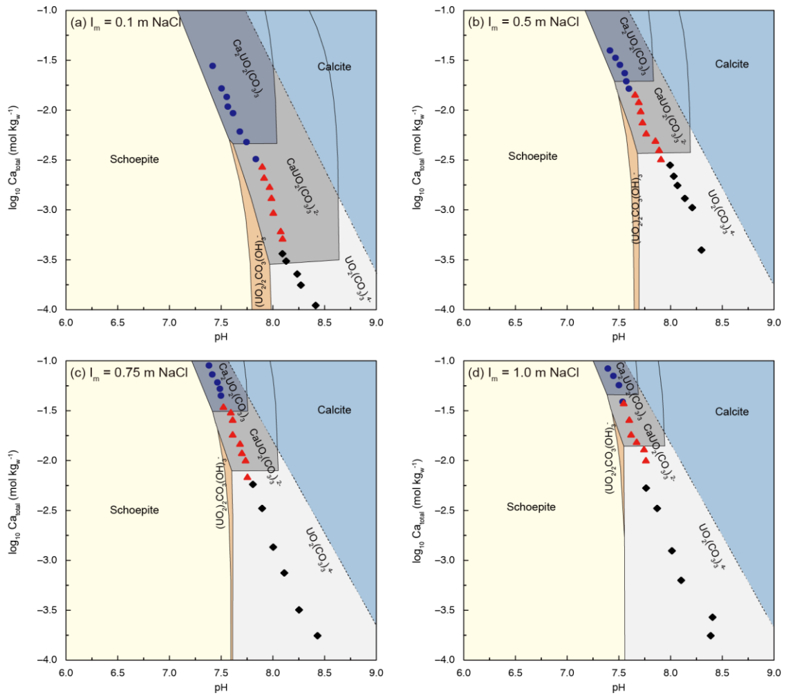
Fig. II - S5 Predominance plots of Ca-UO 2 -CO 3 system at [\text{U(VI)}] = 50 \mu\text{mol kg}_w^{-1} , P(\text{CO}_2) = 10^{-3.5} \text{ atm} and (a) I_m = 0.1 \text{ mol kg}_w^{-1} , (b) I_m = 0.5 \text{ mol kg}_w^{-1} , (c) I_m = 0.75 \text{ mol kg}_w^{-1} , and (d) I_m = 1.0 \text{ mol kg}_w^{-1} \text{ NaCl} . Experimental points giving slopes of 1 and 2 are highlighted with red triangles and blue filled circles, respectively. The black diamond represents the beginning of titration where the binary complexes dominated.
