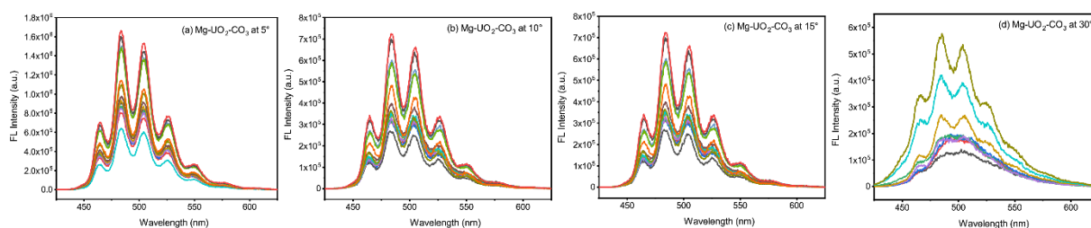
Fig. V - 2 Evolution of luminescence emission spectra during complexation of Mg(II) with UO_2(CO_3)_3^{4-} at different temperature (a)-(d): 5-30°C.
