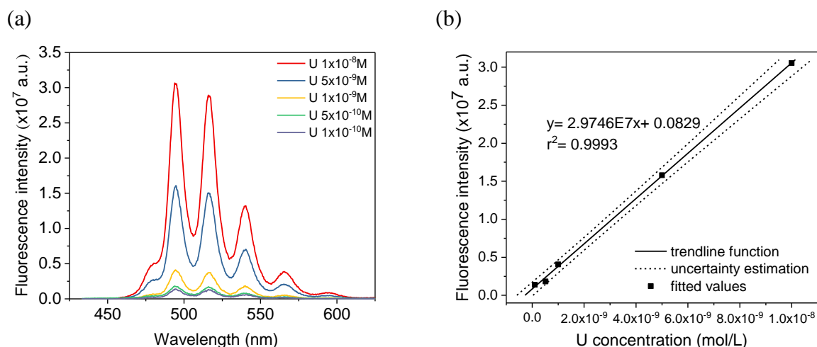
Fig. I - 11 (a) Luminescence spectra of \text{UO}_2^{2+} in 5% \text{H}_3\text{PO}_4 medium at different uranium concentrations from 10^{-8} to 10^{-10} M, recorded at excitation wavelength of 429 nm. (b) Linear dependence of luminescence peak intensities at 485.4 nm on uranium concentration.
