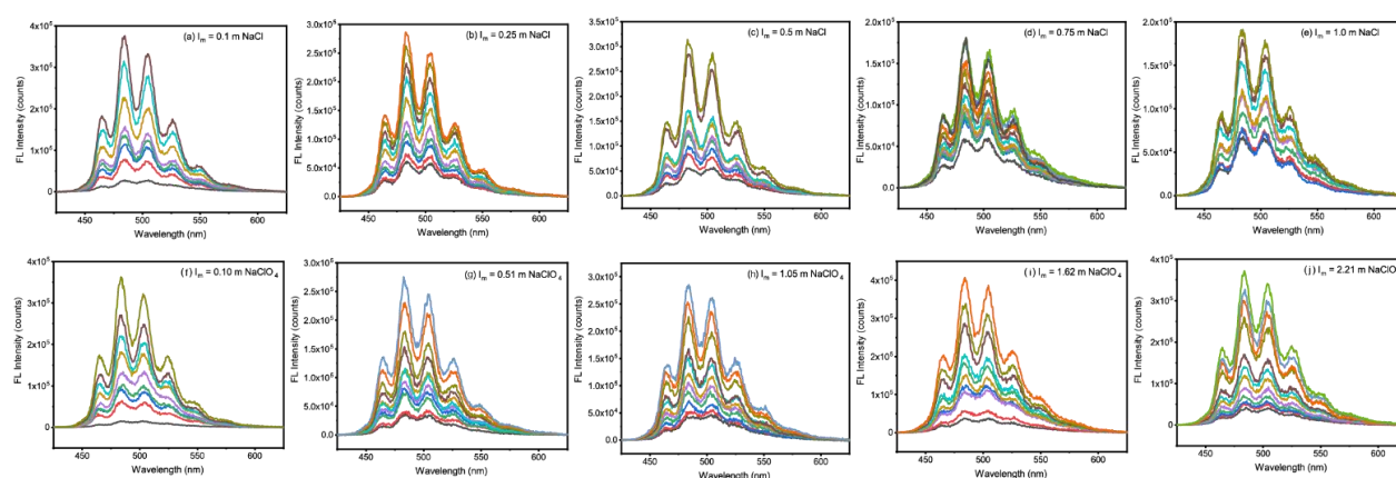
Fig. IV - 3 Graphical representations of luminescence emission spectra on complexation of \text{Mg}(\text{II}) with \text{UO}_2(\text{CO}_3)_3^{4-} at investigated ionic strengths: (a) – (e) I_m = 0.10 - 1.0 \text{ mol kg}_w^{-1} of \text{NaCl} , (f) – (j) I_m = 0.10 - 2.21 \text{ mol kg}_w^{-1} of \text{NaClO}_4 , acquired at D = 25 ns and gate width W = 1\mu\text{s} , number of accumulation is 1000. The aqueous conditions where the \text{MgUO}_2(\text{CO}_3)_3^{2-} complex dominate were listed in Table IV - 4.
