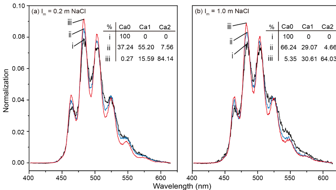
Fig. II -4 Luminescence emission spectra normalized to the same area at D = 25 ns of (Ca-)UO_2-CO_3 species at (a) I_m = 0.2 mol kg_w^{-1} , and (b) 1 mol kg_w^{-1} ; Ca0, Ca1, and Ca2 stand for UO_2(CO_3)_3^{4-} , CaUO_2(CO_3)_3^{2-} , and Ca_2UO_2(CO_3)_3(aq) , respectively.
