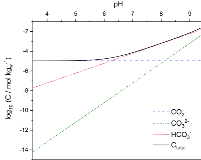
Fig. I - 8 Distribution of carbonate species in equilibrium with air ( P(\text{CO}_2) = 10^{-3.5} \text{ atm} ) as a function of pH. The thick line represents the total dissolved carbonate concentration. (Electrolyte solution: 0.1 \text{ mol kg}_w^{-1} \text{ NaCl} )
