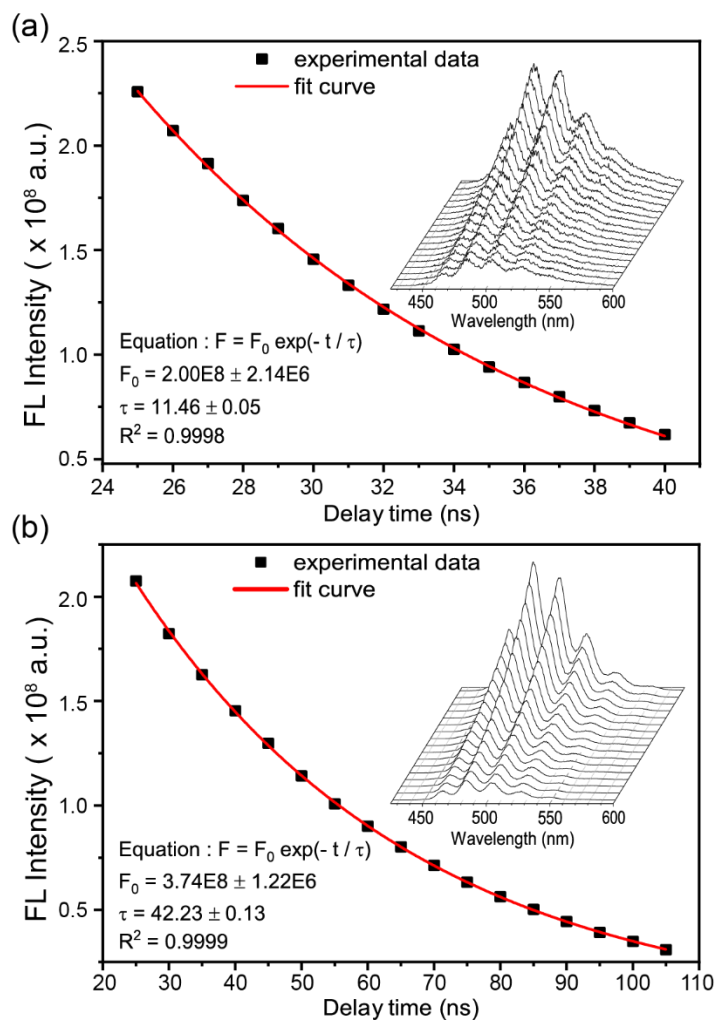
Fig. II - 3 Mono-exponential fits of luminescence intensity decay of (a) UO_2(CO_3)_3^{4-} at [U(VI)] = 50 \mu\text{mol kg}_w^{-1} and pH = 9.0 , and (b) Ca-UO_2-CO_3 complexes at [U(VI)] = 50 \mu\text{mol kg}_w^{-1} , \log_{10}[Ca^{2+}] = -2.06 , pH = 7.60 and I_m = 0.1 \text{ mol kg}_w^{-1} \text{ NaCl} . The insets show the waterfall plots of luminescence emission spectra as a function of delay time.
