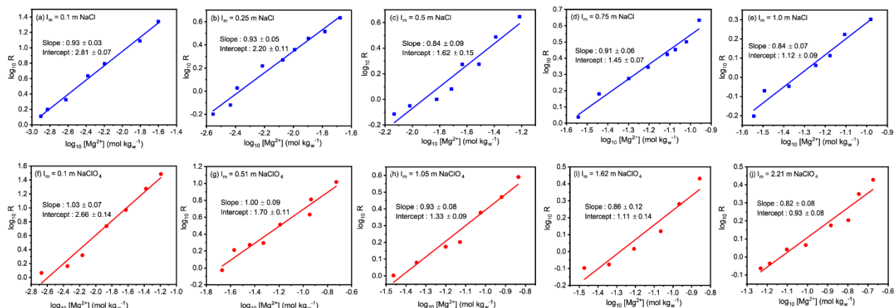
Fig. IV - 1 Plot of logarithmic ratio R as a function of \log_{10}[Mg^{2+}] (mol kg _w^{-1} ) at (a) – (e) I_m = 0.10 - 1.0 mol kg _w^{-1} of NaCl, (f) – (j) I_m = 0.10 - 2.21 mol kg _w^{-1} of NaClO _4 : [U]_{total} = 50 \mu\text{mol kg}_w^{-1} , P(\text{CO}_2) = 10^{-3.5} atm.
