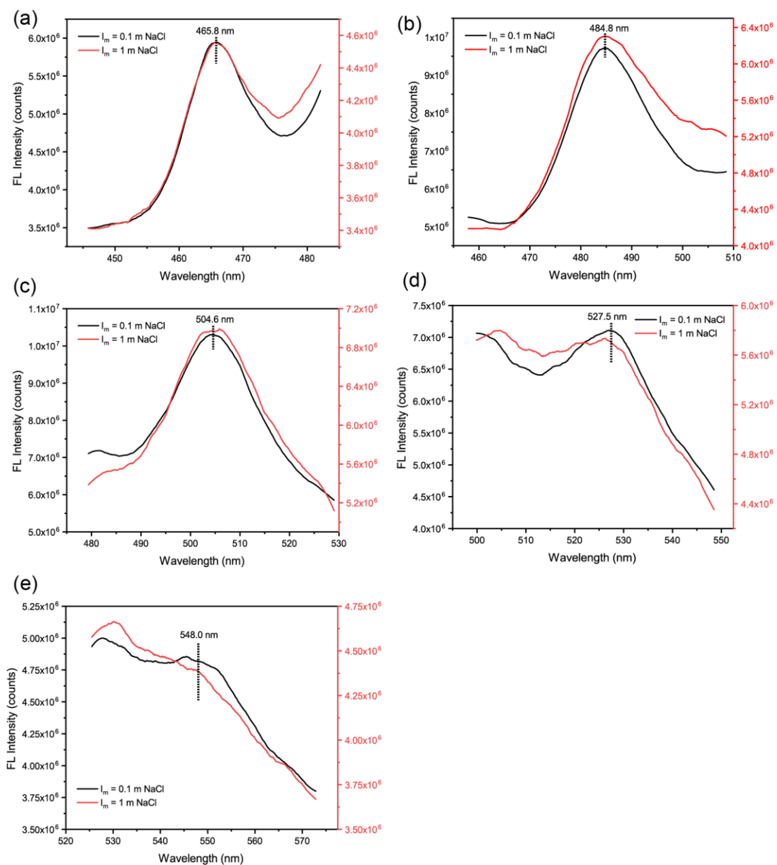
Fig. IV - 5 Measured luminescence emission spectra for each characteristic peak at: (a) 465.8 nm, (b) 484.78 nm, (c) 504.6 nm, (d) 527.5 nm et (e) 548 nm, acquired at delay time at D = 25 \text{ ns} , gate width W = 1 \mu\text{s} and accumulation number 10000 using the 1800 lines \text{mm}^{-1} grating. The spectra were then smoothed for better comparison. The two samples are of U(\text{VI}) = 50 \mu\text{mol kg}_w^{-1} , \text{Mg}(\text{II}) = 0.0042 \text{ mol kg}_w^{-1} , \text{pH} = 7.90 at I_m = 0.1 \text{ mol kg}_w^{-1} NaCl and \text{Mg}(\text{II}) = 0.0442 \text{ mol kg}_w^{-1} , \text{pH} = 7.65 at 1 \text{ mol kg}_w^{-1} NaCl. The peak positions were averaged to be 464.63 \pm 0.32 \text{ nm} , 483.77 \pm 0.29 \text{ nm} , 503.71 \pm 0.33 \text{ nm} , 525.08 \pm 0.80 \text{ nm} and 546.24 \pm 2.21 \text{ nm} in NaCl using the 300 lines \text{mm}^{-1} grating.
