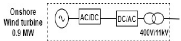
Figure II-7. Overall schematic diagram of wind energy system.
