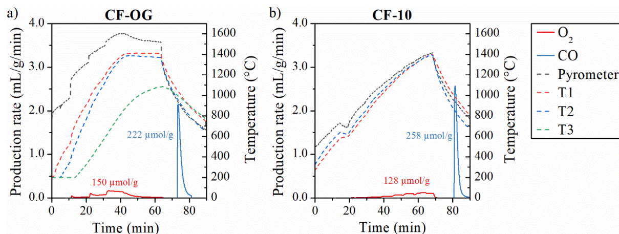
Figure 3-24: O 2 and CO evolution along with the temperature profiles during thermochemical cycling of ceria foams: a) CF-OG (cycle #1) and b) CF-10 (cycle #31), with a reduction at 1400 °C under reduced pressure followed by oxidation starting at 1050 °C under 100 %CO 2
