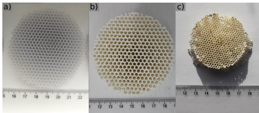
Figure 3-3: a) Ordered polymer template obtained from additive manufacturing, b) ceria impregnated template and c) final ceria structure with ordered-geometry after heat-treatment of b)
