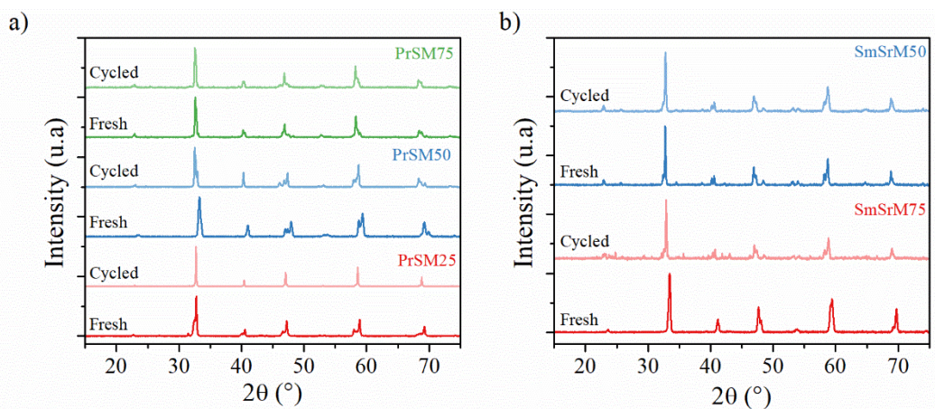
Figure SB-5: XRD patterns of fresh and cycled perovskites: a) PrSrM75, PrSrM50 and PrSrM25 and b) SmSrM50 and SmSrM75 powders
