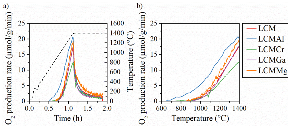
Figure SB-2: O 2 production rate as a function of a) time and b) temperature for lanthanum manganese doped calcium perovskites
