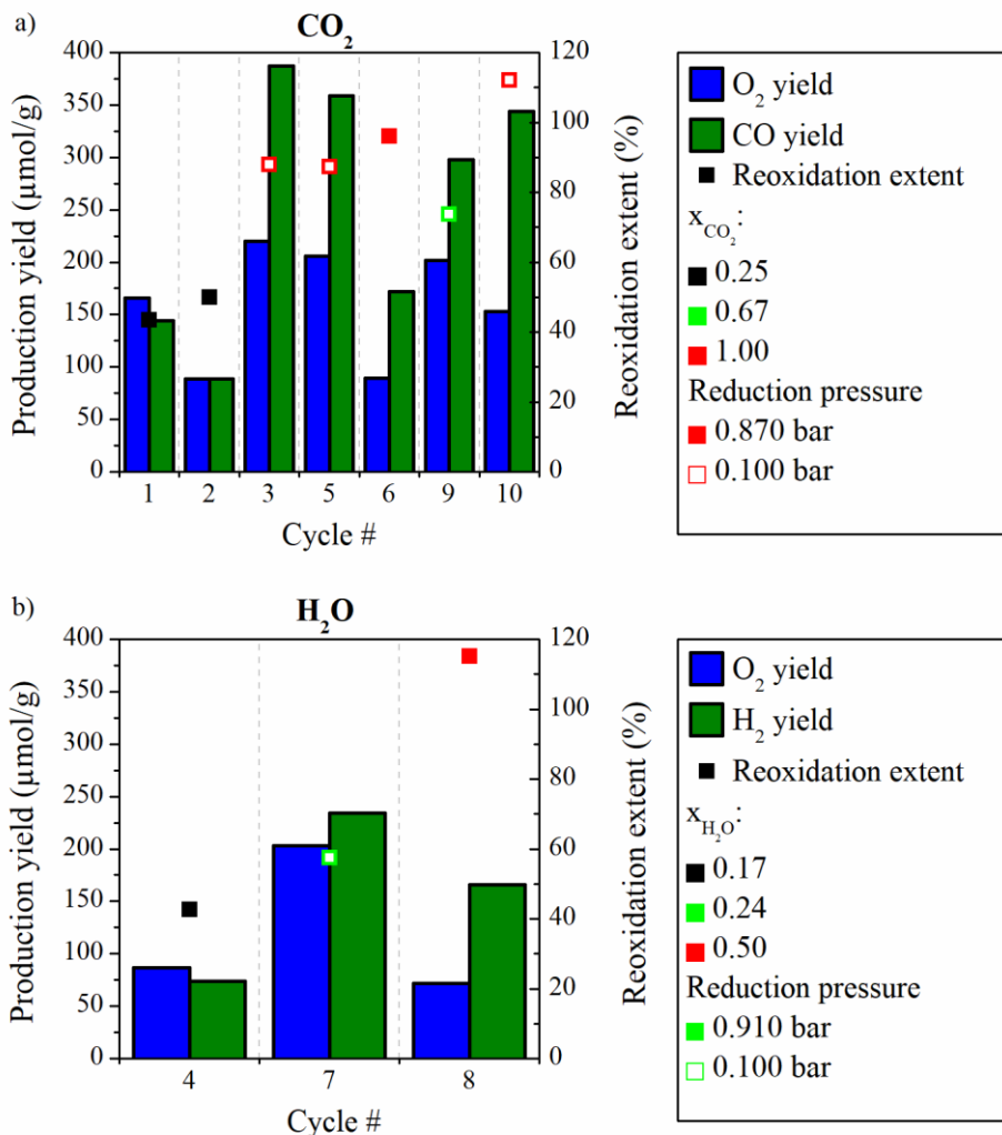
Figure 3-19: Fuel production yields and re-oxidation extents with different operating conditions for a) CO 2 oxidant gas and b) H 2 O oxidant gas for CF-LSMMg; the bar color represents the gas produced, the square color shows the oxidant molar fraction and hollowed symbol indicates a low pressure during the reduction step
