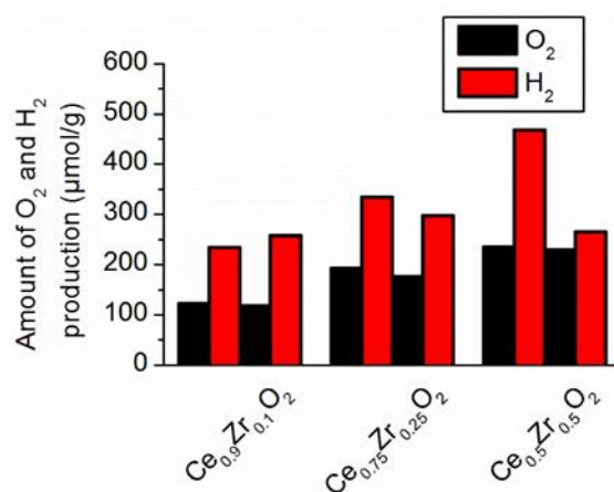
Figure 1-11: \text{O}_2 and \text{H}_2 production during two thermochemical cycles using \text{Ce}_{1-x}\text{Zr}_x\text{O}_2 ( x = 0.1, 0.25 and 0.5 ) with reduction and oxidation temperatures of 1400 °C and 1050 °C, respectively [77].
