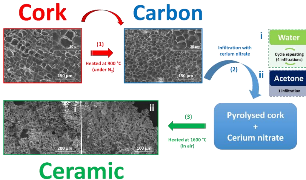
Figure 4-1: Schematic representation of the synthesis protocol for producing cork-derived ceria ecoceramics. Two different synthesis processes were compared, i) using water and ii) using acetone, and SEM images of the two resulting ceria ecoceramics are compared
