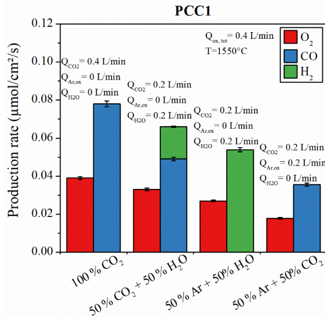
Figure 5-12: O 2 and CO production rates with different compositions of oxidant gas, for PCC1 membrane (conditions #2, 6, 7 and 1)
