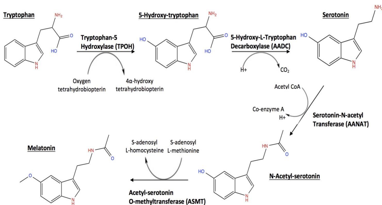
Figure 20: The serotonin pathway to metabolize tryptophan into serotonin and further along into melatonin. Adapted from (Bubenik and Konturek 2011).
