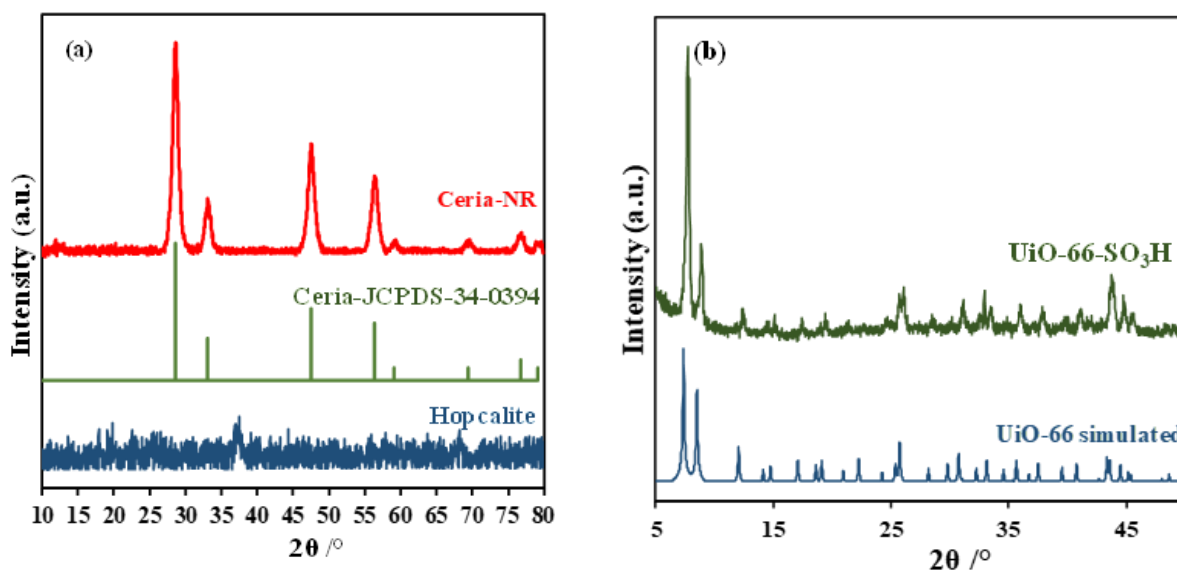
Figure 3.1. XRD patterns of (a): Hopcalite and \text{CeO}_2\text{-NR} , (b): \text{UiO-66-SO}_3\text{H} .
