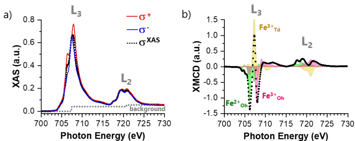
Figure 2.13. Fe L_{2,3} -edges (a) XAS and (b) XMCD spectra for \text{Fe}_3\text{O}_4 acquired at magnetic induction of 2.0 T and at room temperature. Here the raw spectra were normalized to the pre-edge and the background constant to 1 was subtracted. The contributions of each iron species – \text{Fe}^{2+}_{\text{Oh}} , \text{Fe}^{3+}_{\text{Oh}} and \text{Fe}^{3+}_{\text{Td}} – are shown in green, pink and yellow shades, respectively. These curves were simulated using the atomic multiplet theory, as described in Section 2.4 . The dotted gray line depicts the typical “step-like” background (with higher intensity at the L_2 -edge) due to transition to delocalized states.
