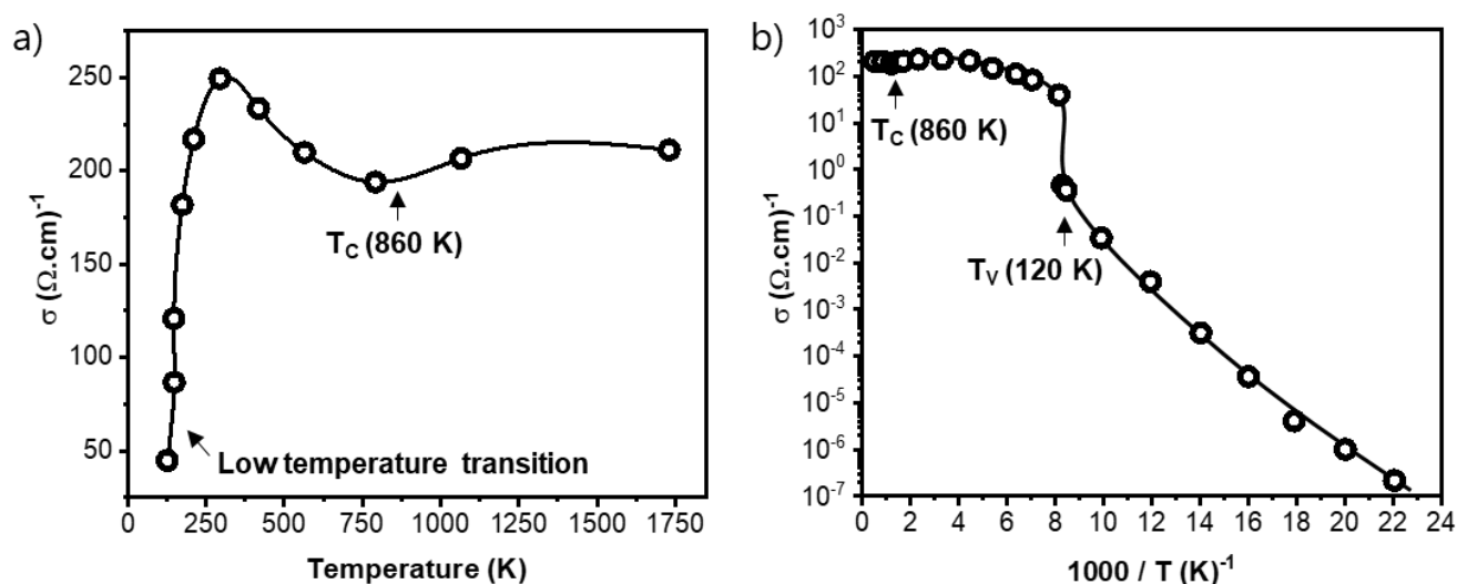
Figure 1.11. Temperature ( T ) dependence on the dc conductivity ( \sigma ) of \text{Fe}_3\text{O}_4 single crystal. The magnetite has several conduction regimes depending on the temperature, as highlighted in (a). The conductivity passes through a maximum at about 350 K and then shows a drop of two orders of magnitude at about 120 K ( T_V ), as verified in (b). Experimental data from Miles et al. [111].
