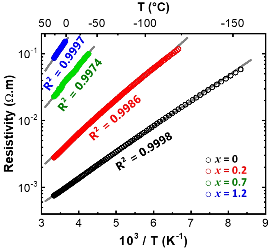
Figure 5.11. Electronic transport behavior in \text{Fe}_{3-x}\text{Cr}_x\text{O}_4 thin films. Herein, the temperature-dependent resistivity ( \rho ) is plotted as Arrhenius curves. According to the coefficient of determination ( R^2 ), reasonably good linear fit (gray straight lines) is found for \ln \rho against 1/T . Color code: x = 0 (black), x = 0.2 (red), x = 0.7 (green) and x = 1.2 (blue).
