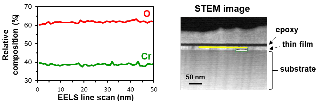
Figure 3.7. At left, Cr and O relative compositions measured using STEM-EELS for 16 nm thick \alpha\text{-Cr}_2\text{O}_3(0001) thin films grown on \alpha\text{-Al}_2\text{O}_3(0001) . At right, STEM images show the position of the horizontal line scan.
