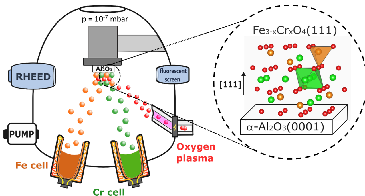
Figure 2.1. Schematic representation of the O-MBE setup for the growth of \text{Fe}_{3-x}\text{Cr}_x\text{O}_4 series on sapphire substrate.
