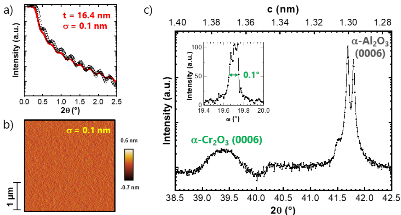
Figure 3.3. Structural characterization of a representative \alpha\text{-Cr}_2\text{O}_3 (0001) grown on \alpha\text{-Al}_2\text{O}_3 (0001) substrate. (a) The thickness of the film, t , is obtained by the fit (red line) of the XRR pattern (black circles) using Parratt’s formulism (see Section 2.2.2 ). The roughness retrieved in the XRR fit ( \sigma_{\text{XRR}} = 0.1 nm) is the same as the one derived from the (b) AFM image ( \sigma_{\text{AFM}} = 0.1 nm). (c) The \theta - 2\theta XRD scan shows the (0006) Bragg peak for \alpha\text{-Cr}_2\text{O}_3 layer ( 2\theta = 39.4^\circ , c = 1.37 nm) and \alpha\text{-Al}_2\text{O}_3 substrate ( 2\theta = 41.7^\circ , c = 1.30 nm). In inset, the rocking curve on the (0006) peak ( \Delta\Omega = 0.1^\circ ) confirms the high crystalline quality of the film.
