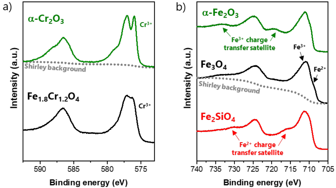
Figure 2.9. Reference (a) Cr and (b) Fe 2p XPS spectra for different chromium and iron oxides. For \alpha - \text{Fe}_2\text{O}_3 and \text{Fe}_2\text{SiO}_4 , \text{Fe}^{3+} and \text{Fe}^{2+} charge transfer satellites are marked with green and red arrows, respectively. For \text{Fe}_3\text{O}_4 , the \text{Fe}^{2+} and \text{Fe}^{3+} contributions are evidenced using black arrows. The Shirley-type background is depicted as dotted gray line.
