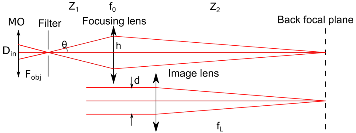
Fig. 3.8 Image generation based on geometrical optic.
