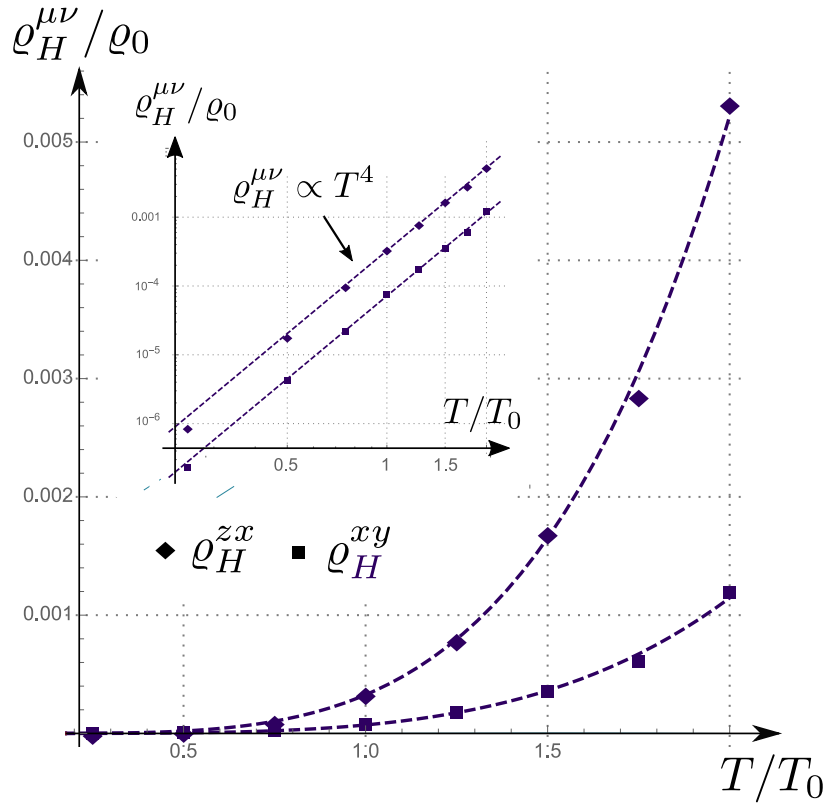
Figure 2.5: Thermal Hall resistivity \varrho_H^{xy} and \varrho_H^{zx} (in units of \varrho_0 = \kappa_0^{-1} with respect to temperature T . The transverse magnetization values (m_0^y, m_0^z) used for computing \varrho_H^{xy} and \varrho_H^{zx} were (0.0, 0.05) and (0.05, 0.0) , respectively. Inset: log-log plot; the scaling behavior is consistent with the analysis presented in the text.
