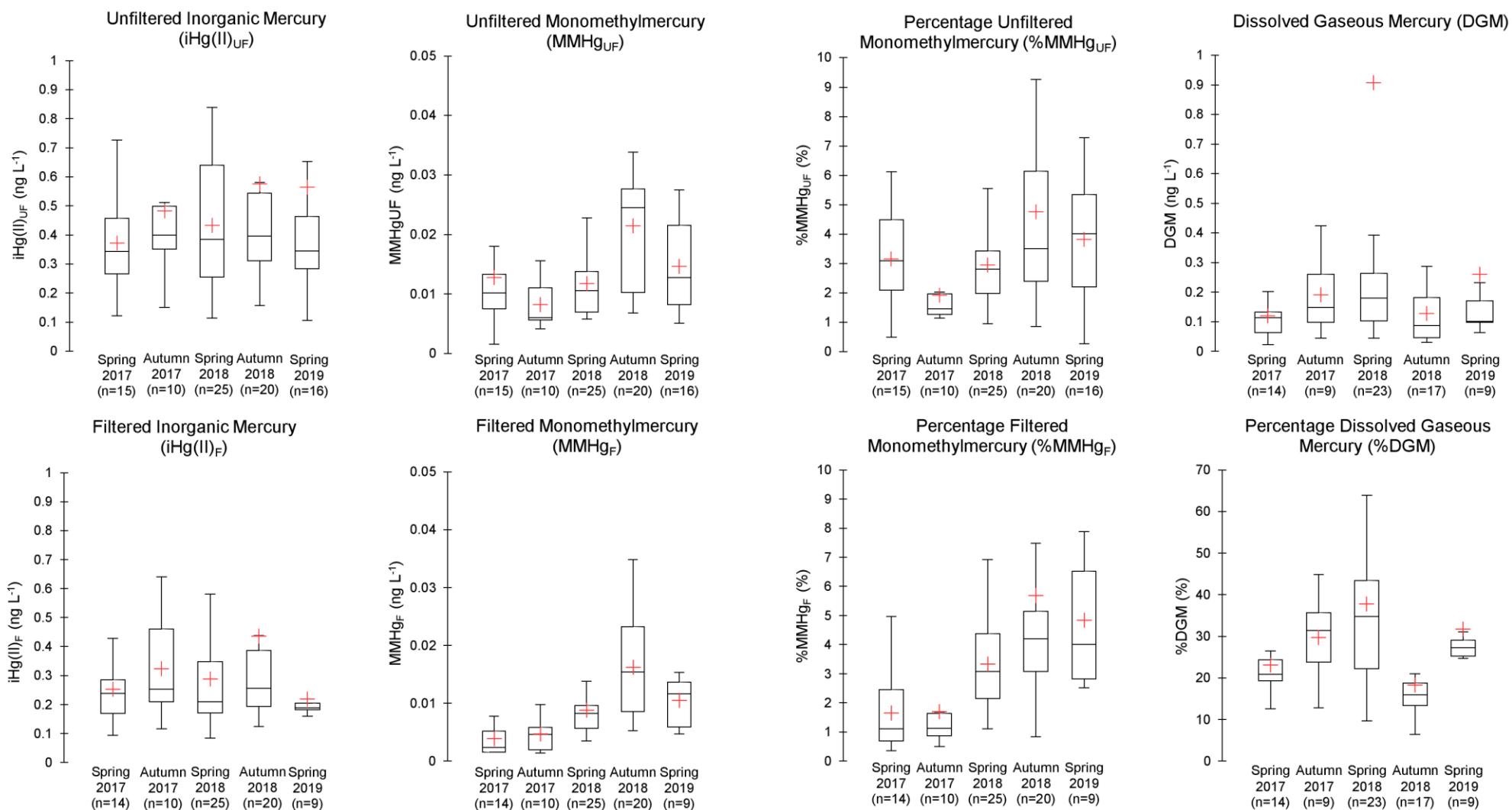
Figure 7-2: Boxplot representations of unfiltered and filtered i\text{Hg(II)} , \text{MMHg} and percentage of \text{MMHg} (calculated as ratio between \text{MMHg} and non-gaseous \text{Hg} ( \text{MMHg} + i\text{Hg(II)} ), and \text{DGM} and percentage of \text{DGM} (calculated as ratio between \text{DGM} and total \text{Hg} ( \text{Hg}_{\text{TOT}} = \text{MMHg} + i\text{Hg(II)} + \text{DGM} )) in subsurface water samples of the 19 studied lakes. Bars indicate 10 th and 90 th percentile, boxes indicate 25 th and 75 th , marks within each box are medians, and red crosses are mean.
