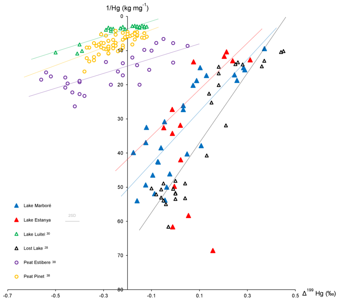
Figure 8-5: \Delta^{199}Hg vs 1/Hg plot for both Lake Marboré and Lake Estanya, together with other lakes [28,30] and peats [38] to highlight some strong linear relationship (dashed lines).
