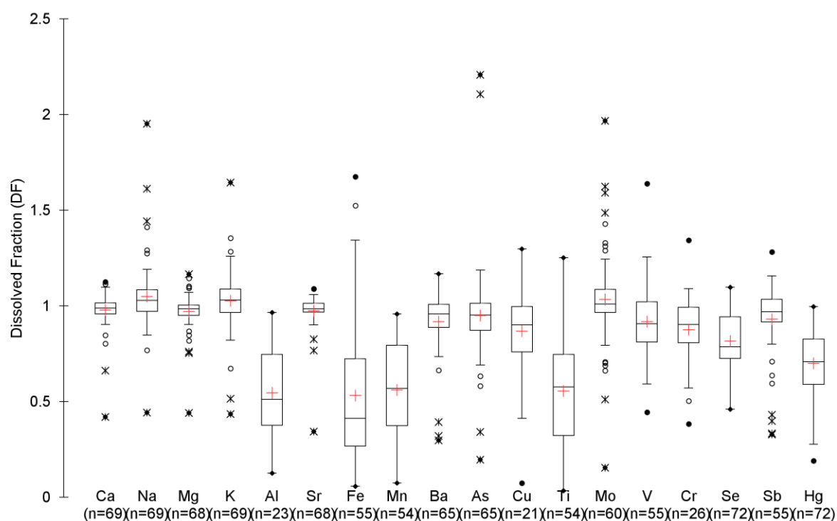
Figure 6-3: Dissolved Fraction (DF) in subsurface water samples calculated for each major, trace and ultra-trace element considered using the results obtained by ICP-MS. Dots are minimum and maximum, white circles are outliers and black crosses are extreme values, bars indicate 10 th and 90 th percentile, boxes indicate 25 th and 75 th , marks within each box are medians and red crosses are mean. For each element, the number n of samples above the LOD for both filtered and unfiltered samples are indicated. Note that Hg corresponds to non-gaseous Hg.
