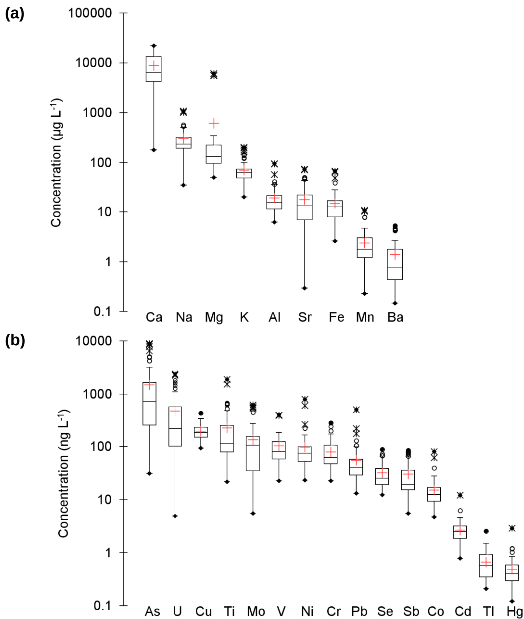
Figure 6-1: (a) Major and trace elements (median concentrations above 1 \mu\text{g L}^{-1} ) and (b) ultra-trace elements (median concentrations below 1 \mu\text{g L}^{-1} ) concentrations in unfiltered subsurface water samples of the 20 studied lakes over the four sampling campaigns. Dots are minimum and maximum, white circles are outliers and black crosses are extreme values, bars indicate 10 th and 90 th percentile, boxes indicate 25 th and 75 th , marks within each box are medians and red crosses are mean. Note that Hg corresponds to non-gaseous Hg.
