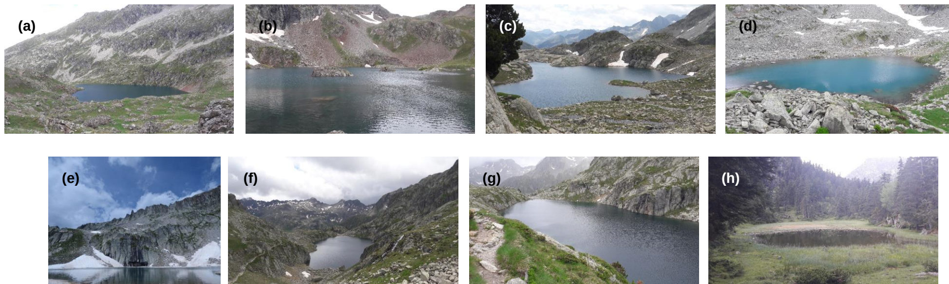
Figure 3-5: Lakes from Cauterets area (Replim1): ARA (a), BAD (b), CAM (c), OPA (d), PEY (e), NER (f), POU (g) and PAR (h)
