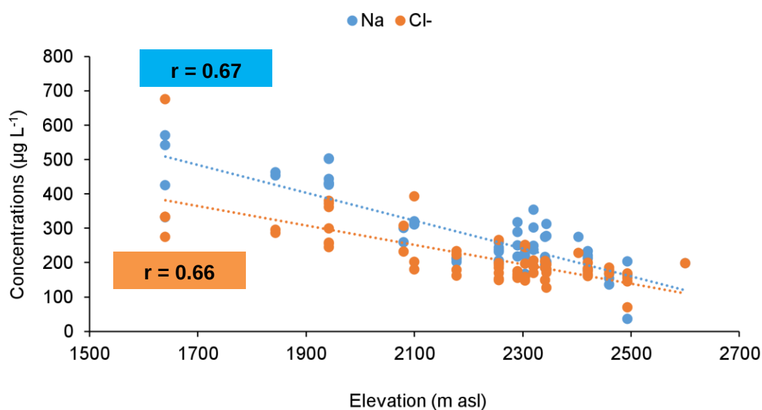
Figure 6-10: Negative correlation between elevation and i) Na and ii) Cl - concentrations (SAB not considered).
