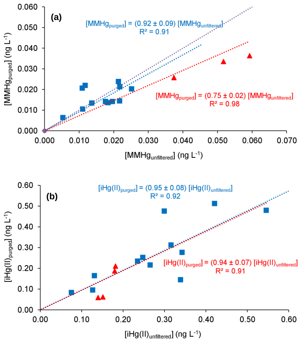
Figure 3-11: Comparison of (a) MMHg concentrations (ng L -1 ) obtained in purged and unfiltered samples (last Lake Gentau depth not shown) and (b) iHg(II) concentrations (ng L -1 ) obtained in purged and unfiltered samples for June 2019 sampling campaign. Square blue points correspond to samples collected in not well oxygenated depths (anoxic water). Red dashed line is the linear regression using all the samples while blue dashed line included only samples from oxic water.
