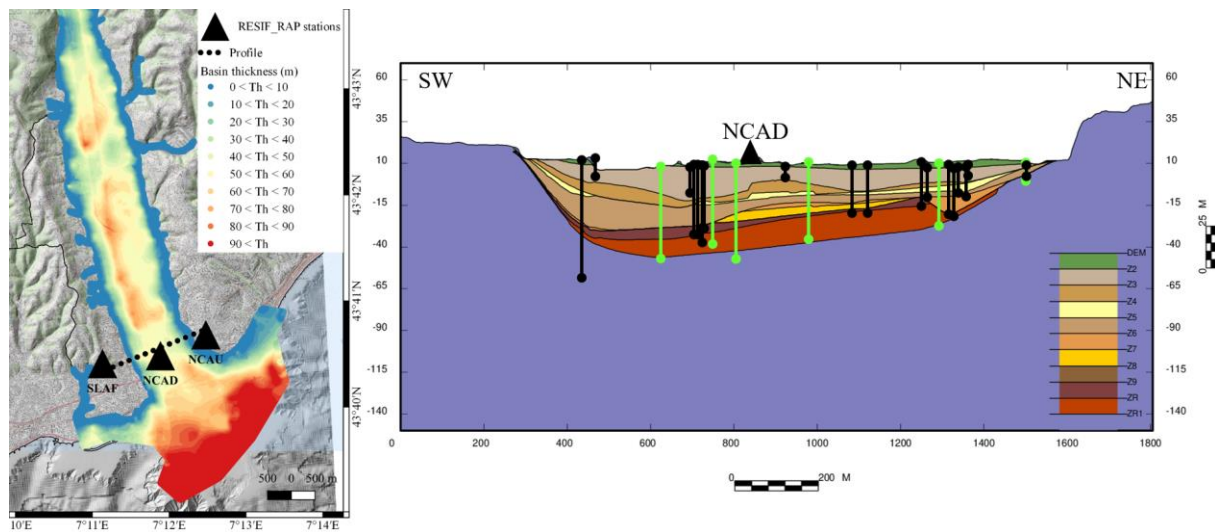
Figure 96: Profile SW-NE in the 3D multi-layered model of the LVV. Different colors represents different layers from the lithostratigraphic profile applied in the LVV (Figure 77). Note that there is one more layer than those defined in the lithostratigraphic profile. It represents the unconstrained layer between the end of the borehole that are not reaching the bedrock and the bedrock depth deduced from ambient vibration data and boreholes reaching the bedrock. The dark lines are boreholes. The green lines are ambient vibration measurements.
