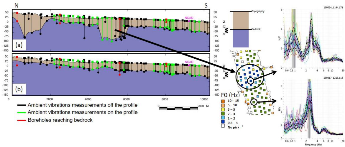
Figure 89: (a) Profile North-South of the geophysical model (based only on ambient vibration data) assuming V_{s,z} constant and taking into account the first peak of mHVSr double peaks. (b) Profile North-South of the geophysical model assuming V_{s,z} constant taking into account the second peak of mHVSr double peaks. Green lines on profiles indicate data located in the middle of the LVV. Black lines on profiles indicate data from a band of 200 m width on both sides of the middle of the valley. Indicated boreholes are located all along the valley.
