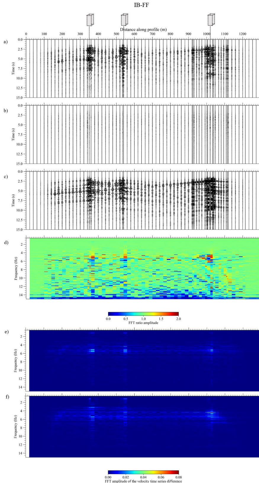
Figure 120: Difference in velocity time series for the transverse (a), longitudinal (b) and vertical (c) components and Fourier spectra amplitude on the transverse component (d) along the SW-NE transverse profile of the basin for the isolated buildings case (IB) compared to the free field (FF) case. (e) and (f) are the Fourier spectra of the difference respectively for the transverse and vertical components. Building positions are schematically indicated at the top of the figure.
