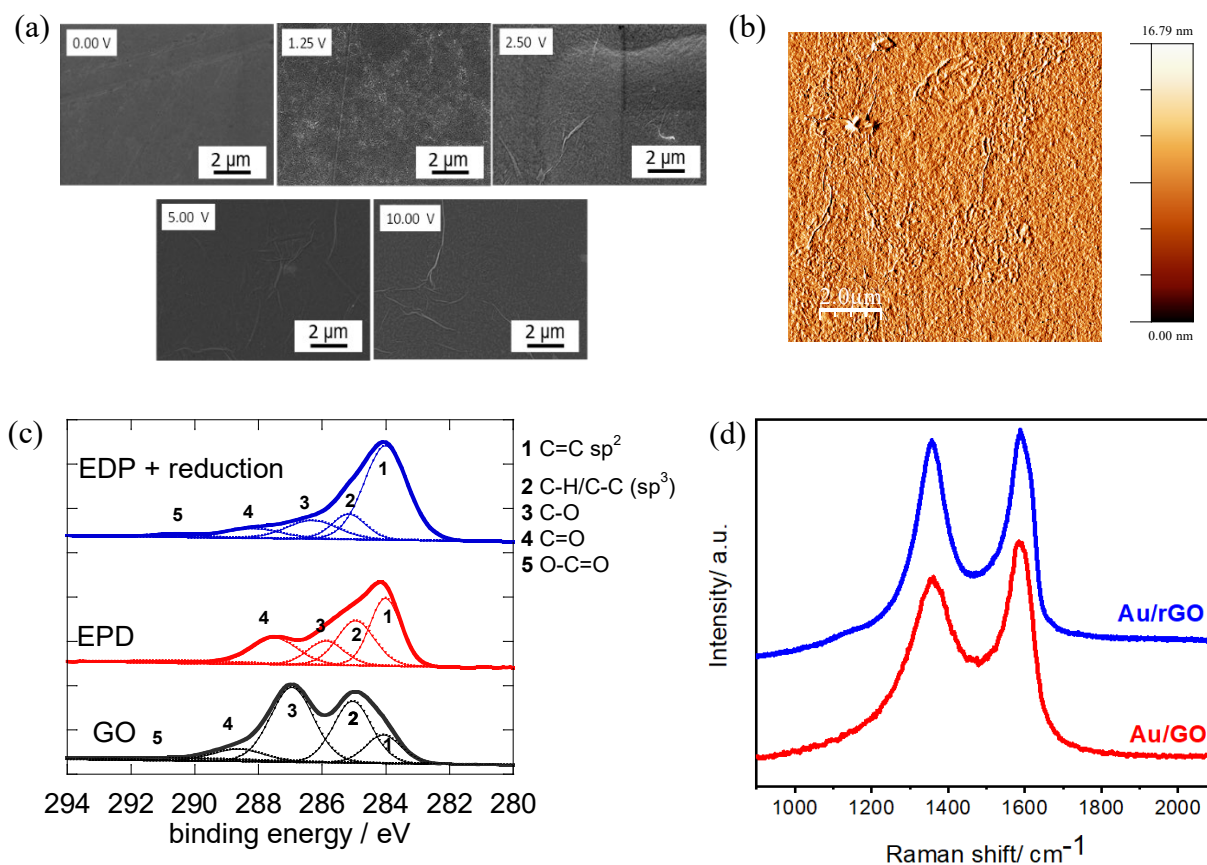
Figure 2.3: Surface characterization of electrophoretically obtained rGO films: (a) SEM images of gold covered electrodes before and after EPD from an aqueous graphene oxide suspension (GO, 1 mg mL -1 ) at different potential biases for 5 min; (b) AFM image of the interface obtained at 2.5 V EPD process after the hydrazine reduction; (c) C 1s high-resolution XPS spectra of initial GO (black), EPD GO (red) and rGO interface (blue); (d) Raman spectra of the EPD film formed at 2.5 V before (red) and after hydrazine reduction (blue).
