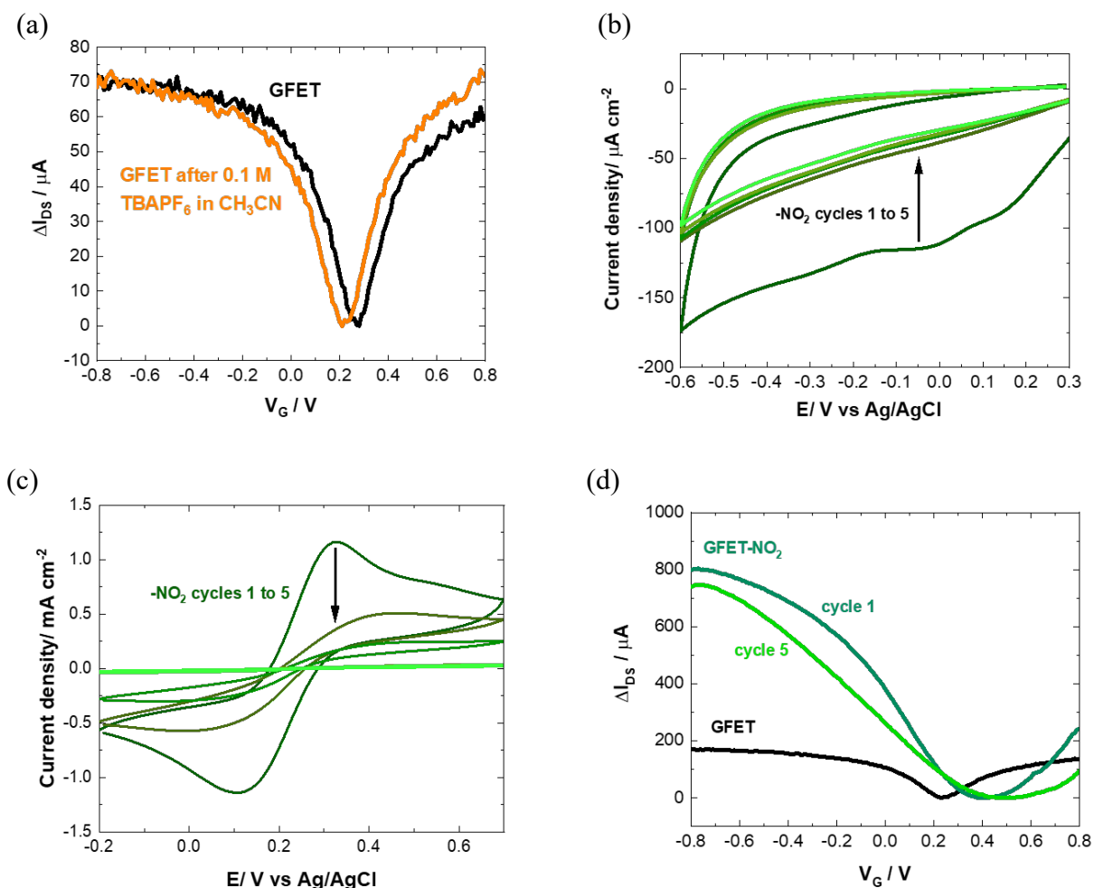
Figure 4.10: Control experiments of diazonium chemistry: (a) I_{DS}V_G of GFET before (black) and after (orange) electrochemical cycling at scan rate of 50 mV s -1 in 0.1 M n-tetrabutylammonium hexafluorophosphate (NBu 4 PF 6 ) in acetonitrile; (b) Electrochemical reduction of a solution of 4-nitrobenzene diazonium tetrafluoroborate (10 mM) in 0.1 M n-tetrabutylammonium hexafluorophosphate (NBu 4 PF 6 ) in acetonitrile via cycling between +0.3 V and -0.6 V (vs. Ag/AgCl) at a scan rate of 50 mV s -1 . The reduction peak is visible at approximately -0.05 V vs. Ag/AgCl; (c) cyclic voltammograms of ferrocenemethanol (1mM/1xPBS) on GFET after each step of the electrochemical grafting of 4-nitrobenzene diazonium tetrafluoroborate; (d) I_{DS}V_G of GFET-NO 2 after 1 and 5 cycles as compared to pristine GFET.
