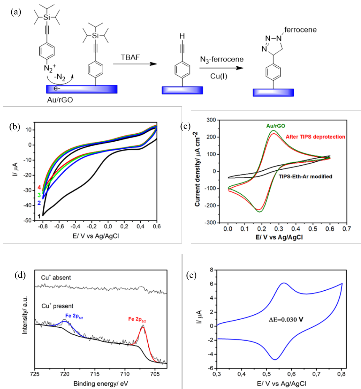
Figure 2.4: Electrochemical grafting of rGO with TIPS and “click” chemistry of ferrocene azide: (a) covalent grafting of EPD rGO electrodes by a silyl-protected diazonium salt followed by tetrabutylammonium fluoride (TBAF)-based deprotection and 1,3-dipolar cycloaddition reaction using azidomethylferrocene as a model compound; (b) electrical reduction of 4-((triisopropylsilyl) ethylenyl)benzenediazonium tetrafluoroborate (TIPS-Eth-ArN 2 + ) with simultaneous rGO surface grafting using cyclic voltammetry from 0.6 to -0.8 V vs Ag/AgCl, scan rate 50 mV s -1 ; (c) cyclic voltammograms in 1 mM ferrocenemethanol in 1xPBS of the Au/rGO interfaces before (green), after diazonium treatment (black) and after the cleavage of the protective group using TBAF (red), scan rate 100 mV s -1 ; (d) high-resolution Fe 2p XPS core-level spectra of ferrocene modified Au/rGO surfaces with and without Cu(I) catalyst during the “click” chemistry reaction; (e) cyclic voltammogram of Au/rGO/Ferrocene modified electrode in acetonitrile/NBu 4 PF 6 (0.1 M), scan rate 100 mV s -1 .
