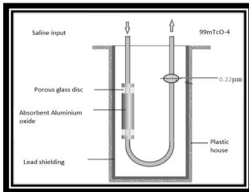
Figure 7 Schematics of the ^{99}\text{Mo}/^{99m}\text{Tc} generator's chromatographic column
