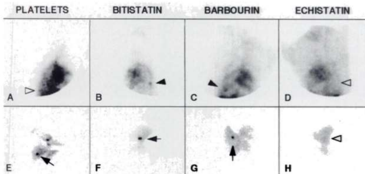
Figure 32 Planar images of dogs' chests ( A-D ) after 3.5 h of radiotracer injection ( ^{99\text{m}}\text{Tc} -HMPAO-labeled autologous platelets or ^{123}\text{I} -disintegrins). Pulmonary emboli are shown by solid arrows, and outlined arrows showed those emboli not visualized through scintigraphy. Ex-vivo images of the lungs from E-H of same animals placed on face of collimator to acquire counts for 20 min. Embolus was not visualized in right lateral view of A using ^{99\text{m}}\text{Tc} -HMPAO-labeled autologous platelets, however clearly seen by ex-vivo lung image of E ; In case of ^{123}\text{I} -bitistatin, embolus was shown in both views of B and F ; In case of ^{123}\text{I} -barbourin, embolus was seen both in C and G ; In case of ^{123}\text{I} -echistatin, embolus was not seen in both views of D and H . Reproduced from research originally published in JNM , knight et al. 1996 [288].
