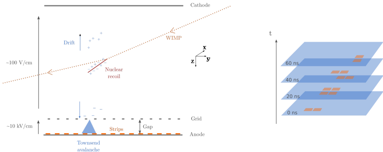
Figure 4.1: Schematic of the MIMAC detection principle. Left: description of an event. Right: the reconstruction of the track in 3D from the pixelated anode measurements.
