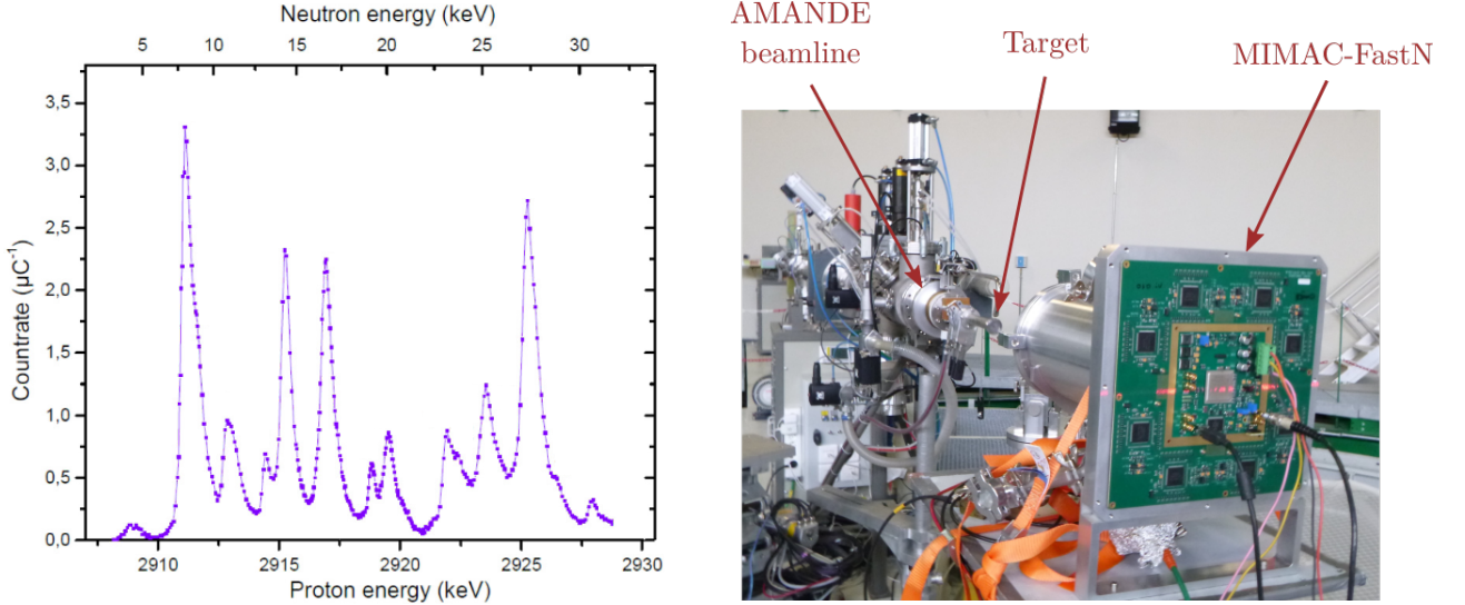
Figure 5.18: Left: the relative neutron fluence rate as a function of the incident proton energy. The fluence is expressed as the count rate in a Bonner sphere assumed to have a flat response in the neutron energy region, enabling comparison between the resonance peaks. Figure adapted from [336].
