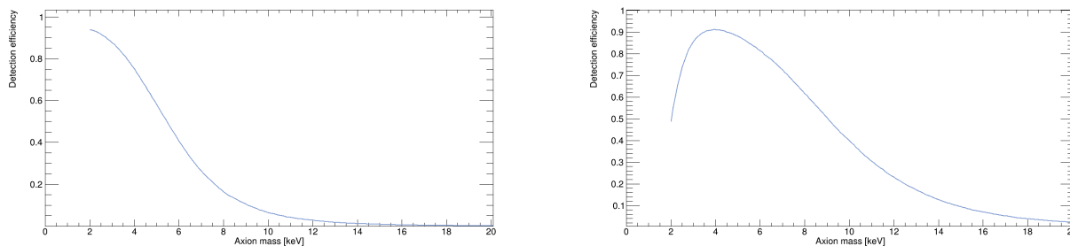
Figure 9.7: Monte-Carlo simulation of the a \rightarrow \gamma\gamma detection efficiency in a 1 \text{ m}^3 MIMAC detector as a function of the axion mass. Left: the Mimac gas at 50 mbar. Right: 95% \text{C}_3\text{F}_8 + 5% \text{i-C}_4\text{H}_{10} at 100 mbar.
