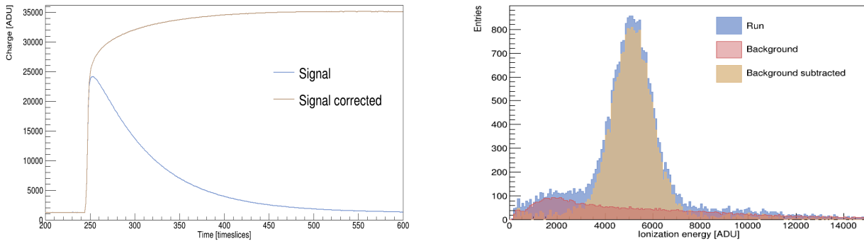
Figure 7.4: Examples of the treatment applied to the data. Left: correction of the ballistic deficit on the measured signal by applying the procedure described in [315]. Right: background subtraction for 1.5 keV electrons.
