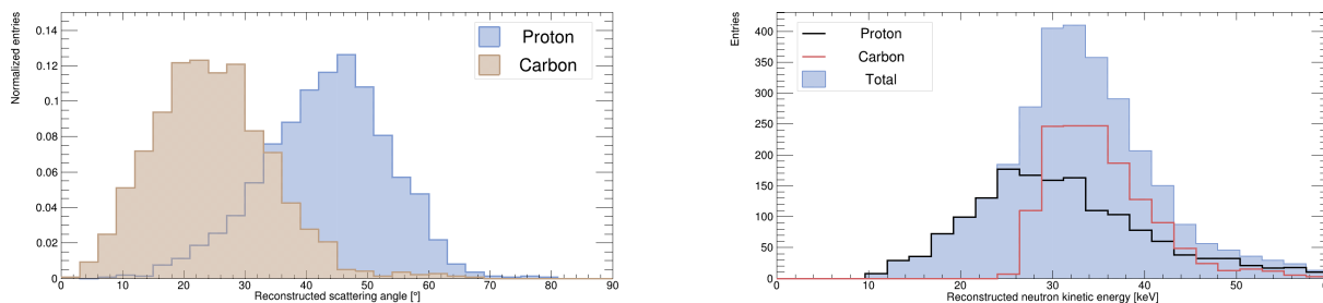
Figure 8.15: Angular distribution (left) and neutron energy spectrum (right) reconstructed from proton and carbon recoils for the AMANDE 27 keV experiment by using the method on the anode. The IQF of proton has been measured whereas the IQF of carbon is scaled from SRIM thanks to a normalization factor determined from the difference between simulated and measured IQFs for proton.
