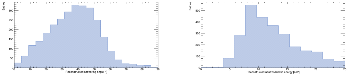
Figure 8.17: Angular distribution (left) and neutron energy spectrum (right) reconstructed from proton recoils for the AMANDE 8 keV experiment by using the method on the anode.
