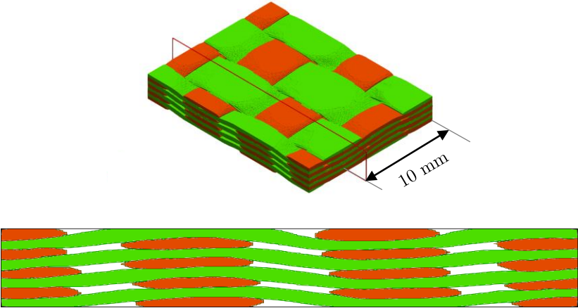
Figure 1.22. Position and cross-sectional observation of the textile geometry along warp tows.
