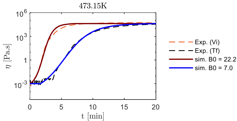
Figure 2.26. Viscosity simulation at 473K compared to some experimental measurement.
