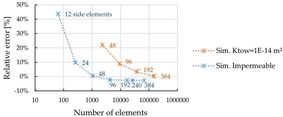
Figure 1.16. Simulation effective permeability error with relation to the number of elements in the mesh with a quasi-impermeable zone (orange) or an impermeable zone (blue).
