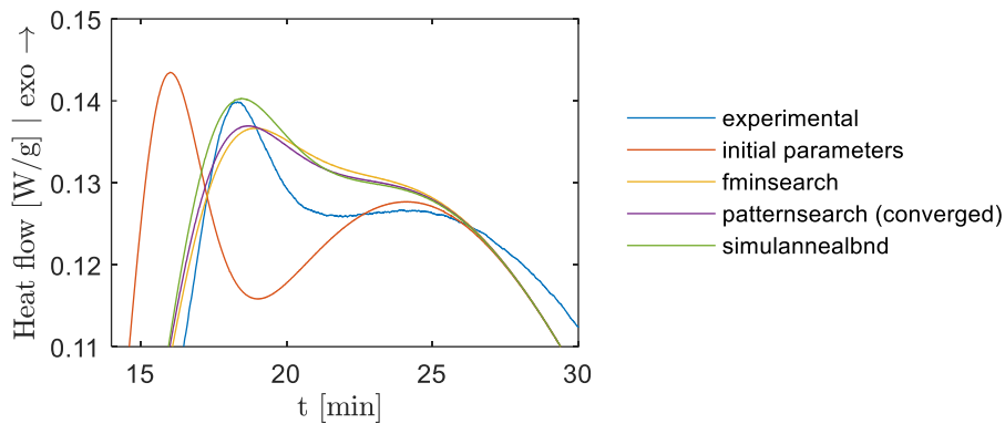
Figure 0.3 Comparison of heat flow curves between initial parameters, optimized parameters by fminsearch, patternsearch and simulannealrnd, and experimental measurement. a/ shows the whole measurement, b/ zooms in the area of interest
