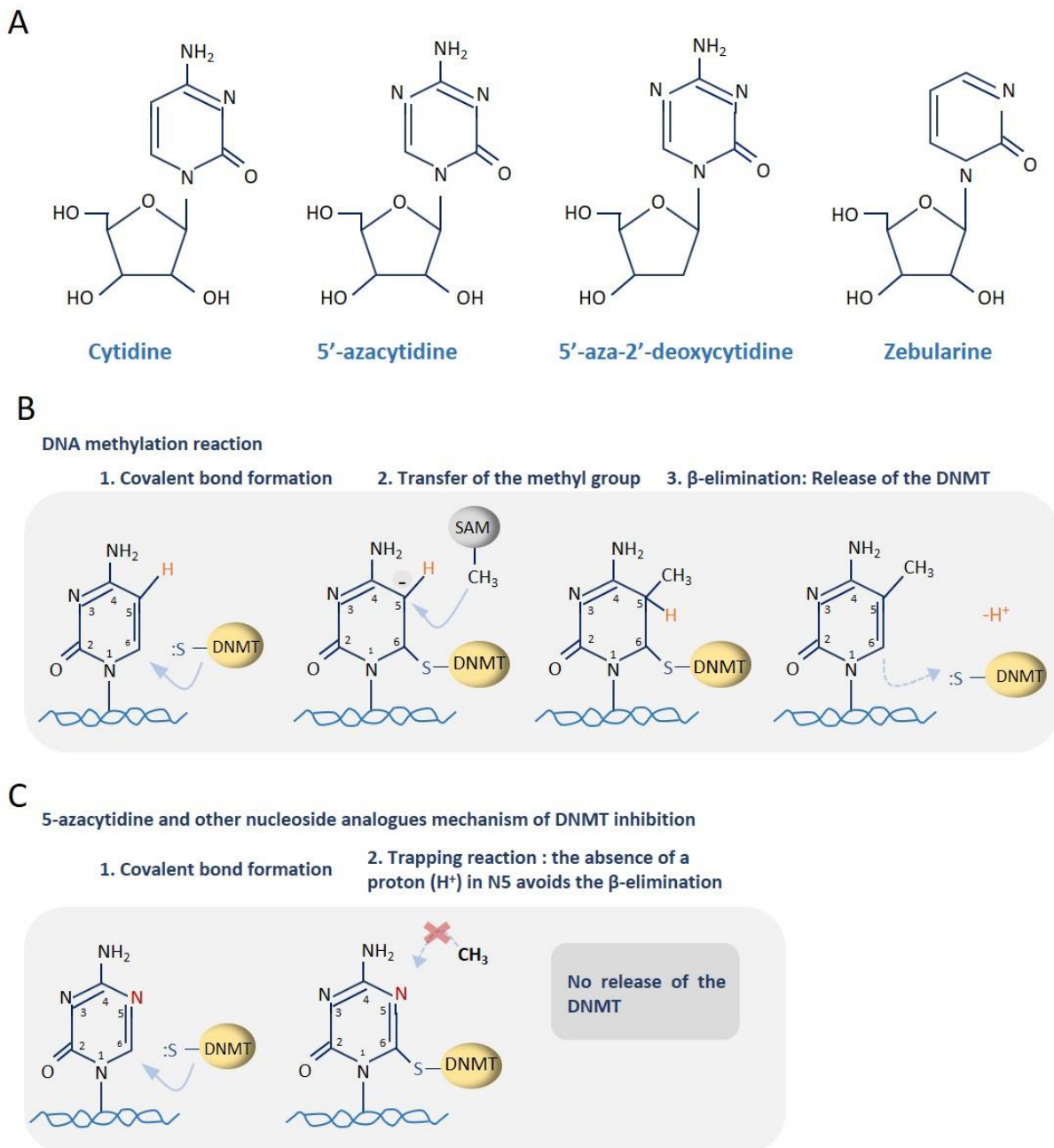
Introductory Figure 11. DNMT inhibition by cytosine analogues.
