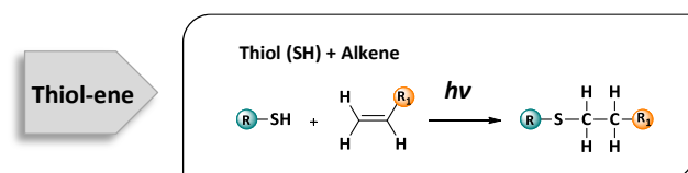
Figure 7. Photoinitiated thiol-ene reaction scheme. In the scheme, the symbols R and R 1 refer to any substituent.
