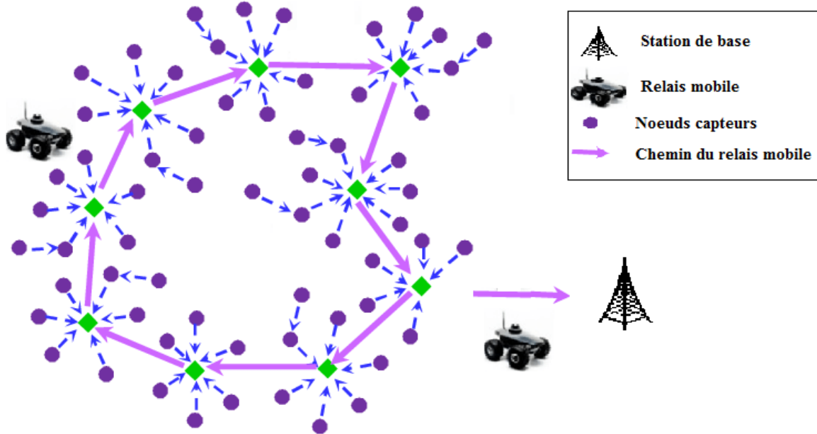
FIGURE 2.9 – Relais mobile
