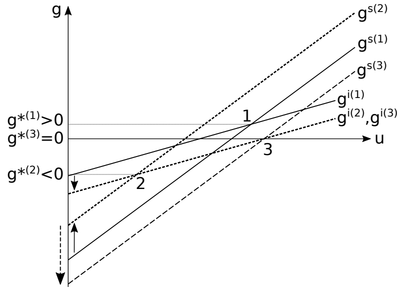
Figure 1.7: Short and medium-run macroeconomic effects of an increase in the tax rate on capital in an extended neo-Kaleckian model.
