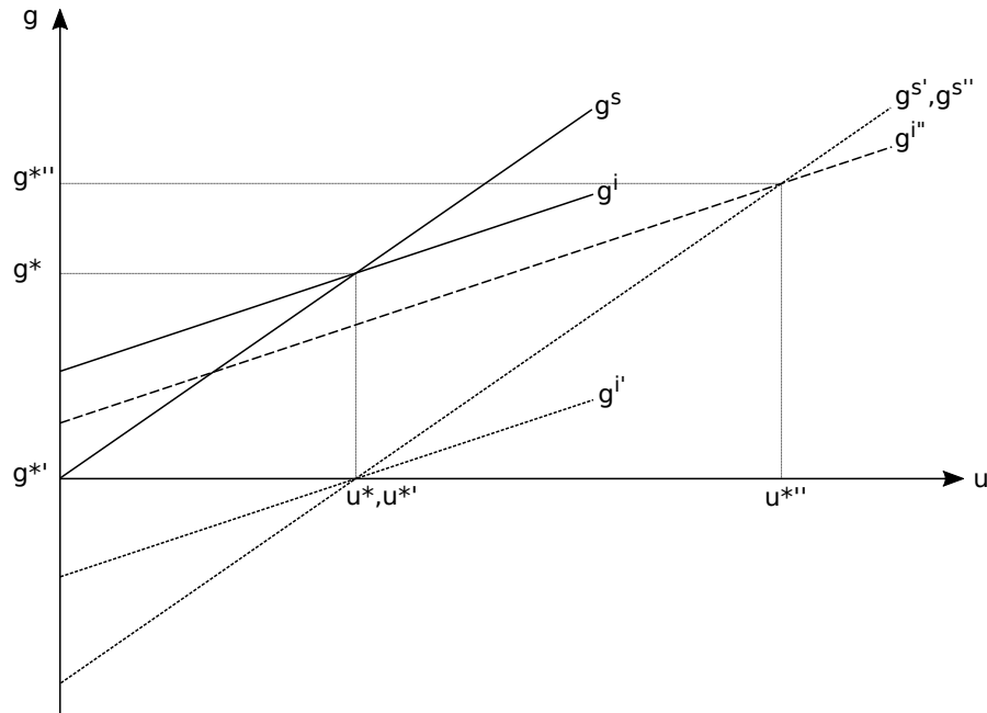
Figure A.1: Change in the equilibrium rates of accumulation and of capacity utilisation when the rate of capital depreciation is introduced.
