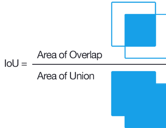
Figure 7.2: Visual example of IoU
