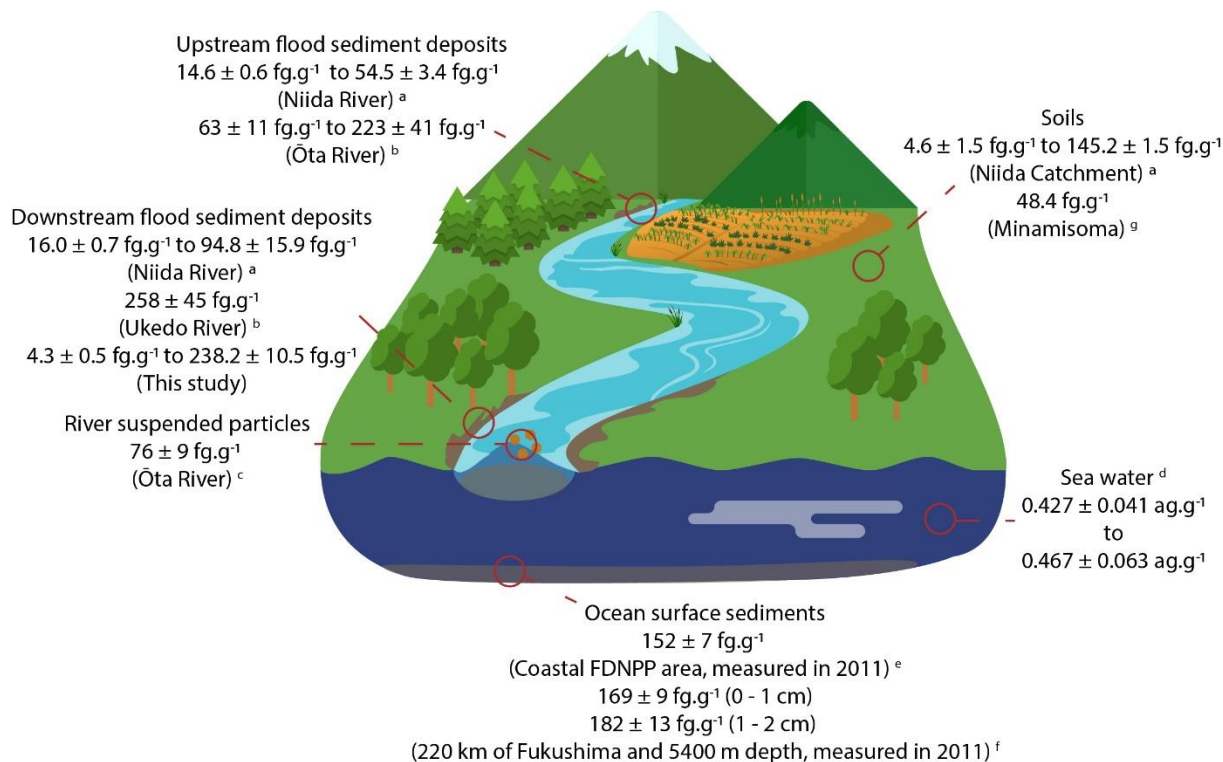
Figure III-2: Sketch illustrating the Pu concentration variations (all values were decay-corrected to March 2021) along the continent-to-ocean continuum. a. (Jaegler et al., 2018) ; b. (Evrard et al., 2014) ; c. (Cao et al., 2016) ; d. (Men et al., 2018) ; e. (Oikawa et al., 2015) ; f. (Bu et al., 2015b) ; g. (Schneider et al., 2013).
