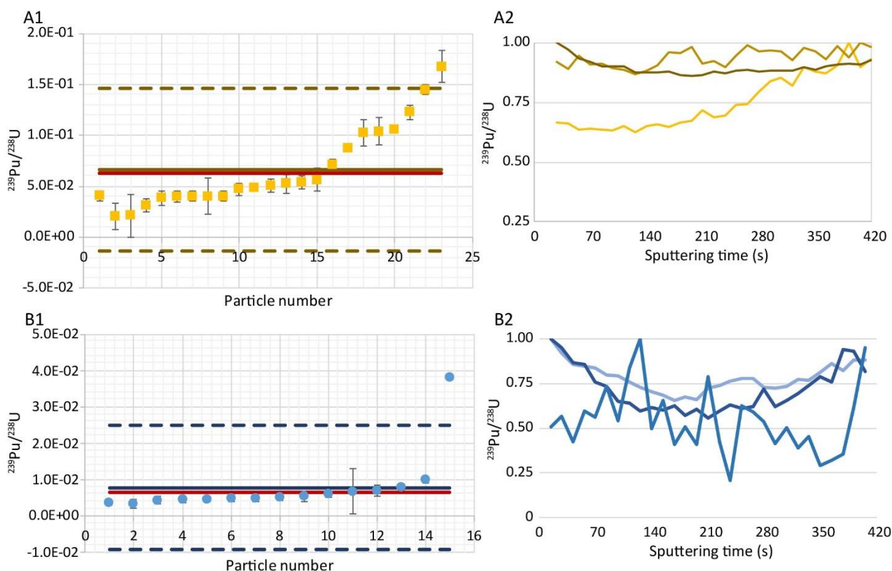
Figure V-5: ^{239}\text{Pu}/^{238}\text{U} isotopic ratios measured in individual particles from (A 1 ) UKMOX-010 sample (yellow squares), and (B 1 ) UKMOX-100 sample (blue points). Individual expanded uncertainties are given with a 95% confidence level. The red line corresponds to the reference value. The yellow and blue lines correspond to the averages of the measured ratios for both samples. The coloured dashed lines correspond to the expanded uncertainties on the average ratio. ^{239}\text{Pu}/^{238}\text{U} isotopic ratios (normalized to the highest ratio) plotted against the sputtering time for three UKMOX-010 particles (A 2 ), and for three UKMOX-100 particles (B 2 ).
