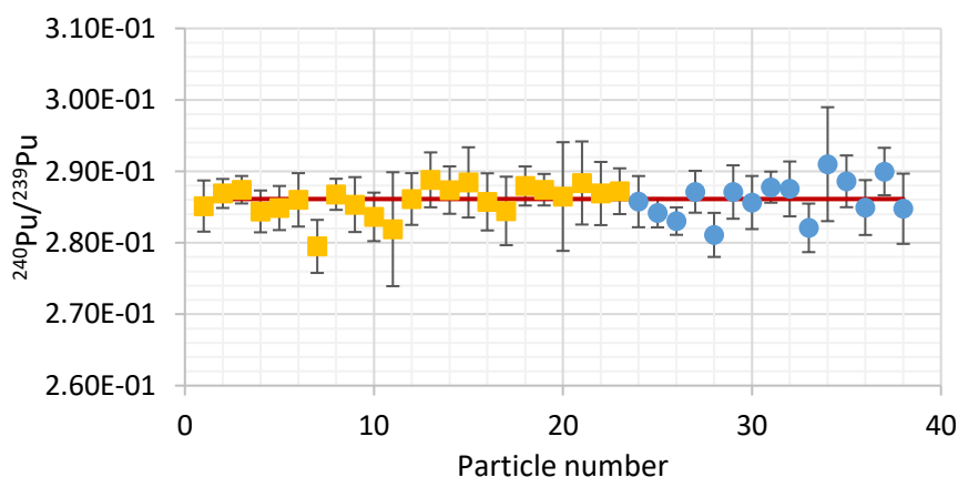
Figure V-3: ^{240}\text{Pu}/^{239}\text{Pu} isotopic ratios measured for individual UKMOX-010 (yellow squares) and UKMOX-100 (blue points) particles. Expanded uncertainties are given with a 95% confidence level. The red line corresponds to the reference value.
