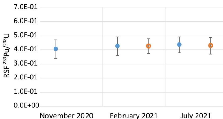
Figure V-4: Average RSF ^{239}Pu/^{238}U measured with the ^{235}U/^{239}Pu (blue point) and with the ^{236}U/^{240}Pu (yellow circles) radio-chronometers. Expanded uncertainties are given with a 95 % confidence level. ^{236}U/^{240}Pu isotopic ratio was not measured during the November 2020 analytical session.
