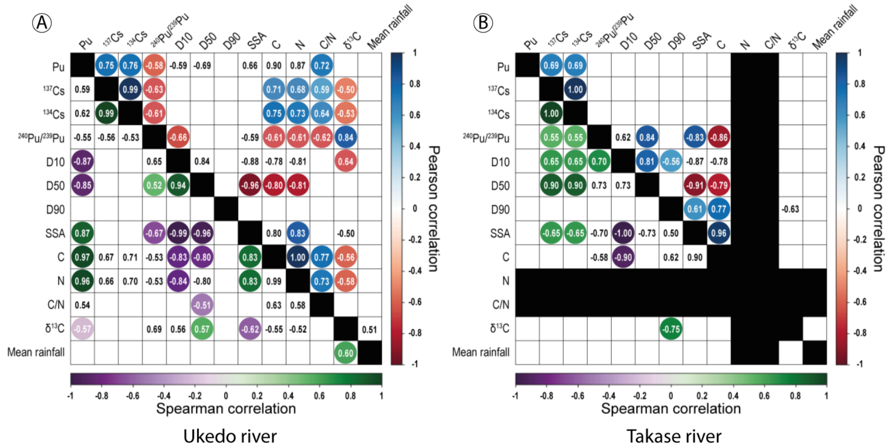
Figure III-5: Significant Pearson (linear; upper part) and Spearman (non-linear; lower part) correlation matrices between radionuclide and sediment properties above 0.5, for (A) Ukedo river (n = 12) and (B) Takase river (n = 10). The highest correlation and anti-correlation value between both modes (i.e., linear and non-linear) are indicated with a coloured circle.
