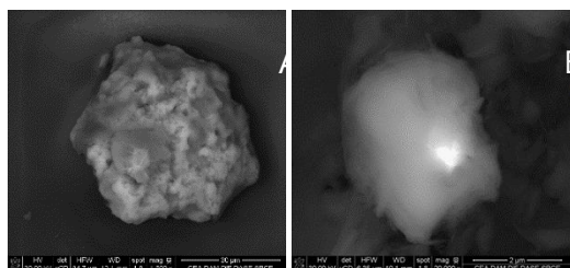
Figure 64: SEM observation of microparticles containing uranium from a Fukushima sediment sample (Okuma 7). A.
