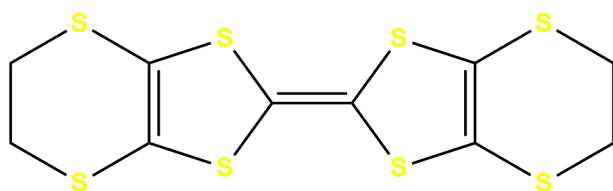
BEDT-TTF
