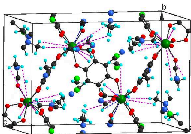
Figure 2.2. Unit cell of the compound 1 showing the H-contacts between \text{Yb}^{\text{III}} and the C-H oscillators, responsible of the quenching of lanthanide emission. Pink dotted lines are d(\text{Ln}^{\text{III}} \cdots \text{C-H}) within 4-5 Å and blue dotted line corresponds to d(\text{Ln}^{\text{III}} \cdots \text{C-H}) within 3-4 Å.
