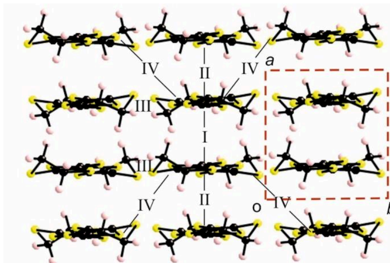
Figure 5.9. Donor layer of the salt 1 where the four different intermolecular interactions are labeled.
