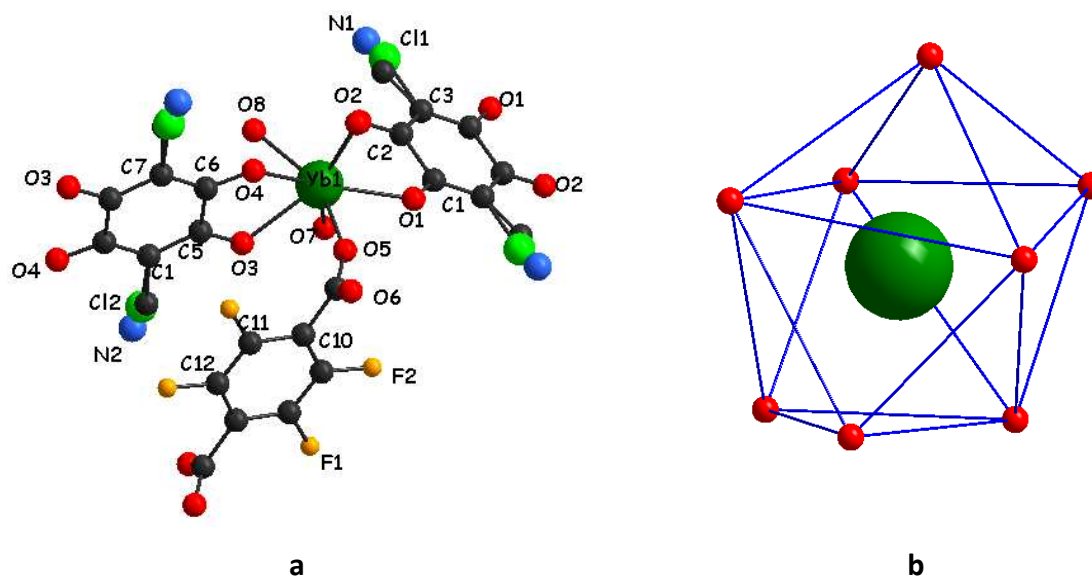
Figure 3.5. (a) The coordination environment of \text{Yb}^{\text{III}} centres in 3 with atom labelling scheme. Solvent molecules are omitted for clarity. (b) trigonal dodecahedron geometry of \text{Yb}^{\text{III}} centre in 3 .
