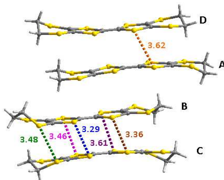
Figure 6.4. S...S contacts (Å) less than the sum of the van der Waals radii (3.65 Å) :S4A-S28D 3.62, S16B-S24C 3.48, S13B-S21C 3.46, S14B-S22C 3.29, S11B-S19C 3.61, S12B-S20C 3.36.
