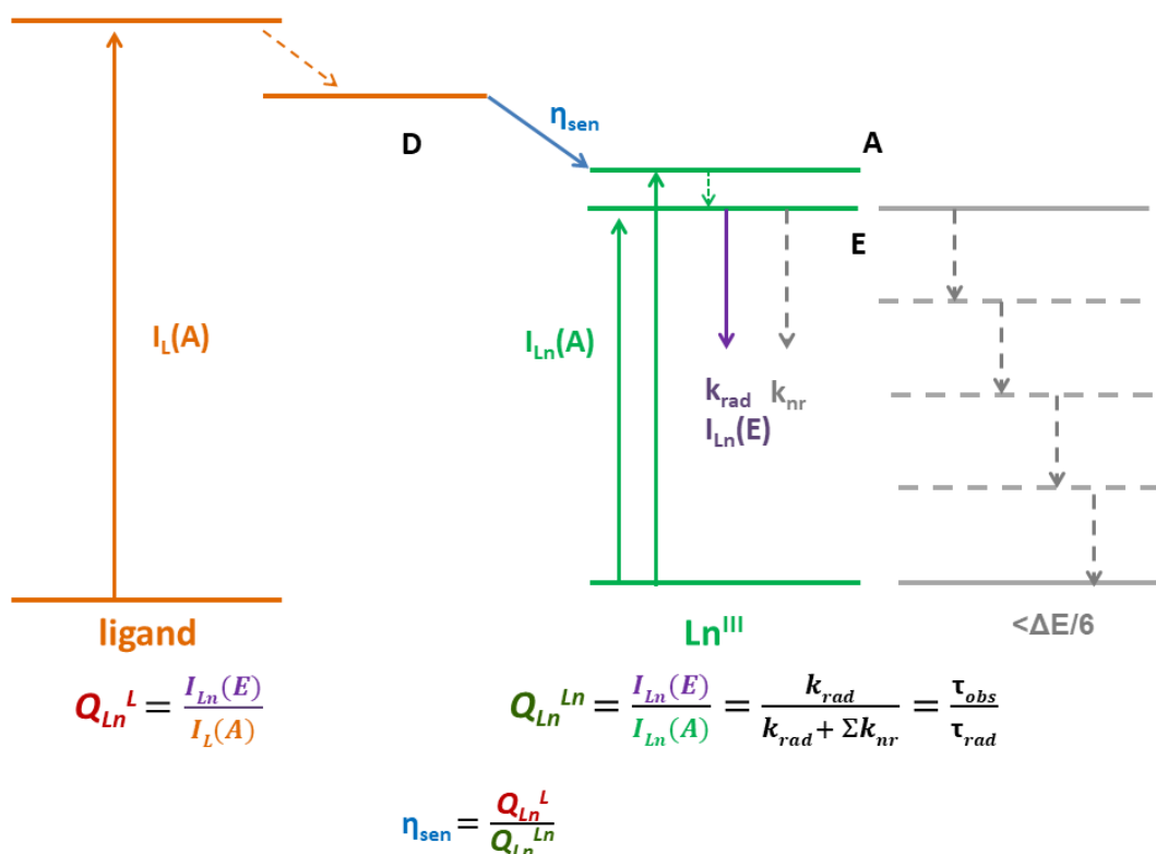
Scheme A3.2: Simplified energy diagram of sensitized luminescence. A = absorption, E = emission, D = donor state. Reprinted from Ref. 1
