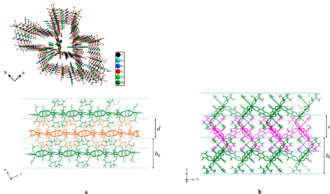
Figure 3. Perspective view of 1 in the b – c plane (top). View of 2D layers showing the thickness of the first monolayer ( h_0 ) and interlayer distance ( d ) in (a) 1 and (b) 3 .
