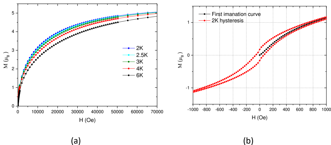
Figure 1.8. (a) Isothermal magnetization of 1 at different temperatures and (b) magnetic hysteresis loop at 2K.
