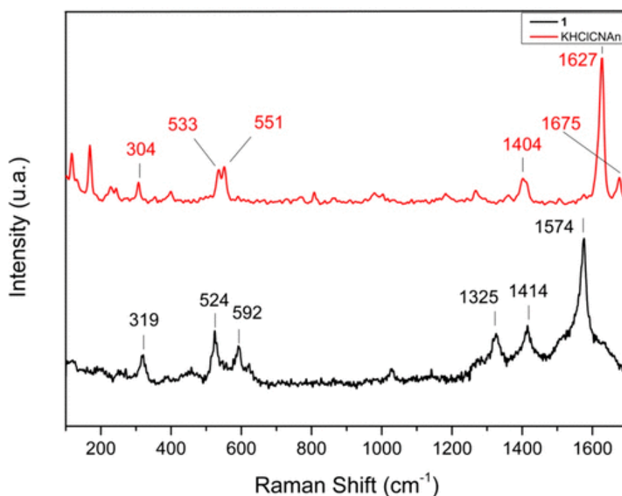
Figure 1.4. Comparison of Raman spectra of 1 and the KHClCNAn ligand, performed at room temperature with a He-Ne laser ( \lambda = 632,81 nm) and a Nd:YAG ( \lambda = 1064 nm), respectively.
