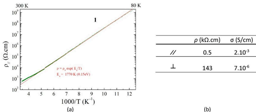
Figure 1.10. (a) Electrical resistivity \rho_{\parallel} plotted as \log \rho_{\parallel} versus the inverse temperature, measured with a 4V voltage applied in the ab plane. The red line is the fit to the data with the law \rho = \rho_0 \exp(E_a/T) giving the activation energy E_a . (b) Room-temperature resistivity ( \rho ) and conductivity ( \sigma ) values measured along ( \parallel ) and perpendicular ( \perp ) to the 2D layers.
