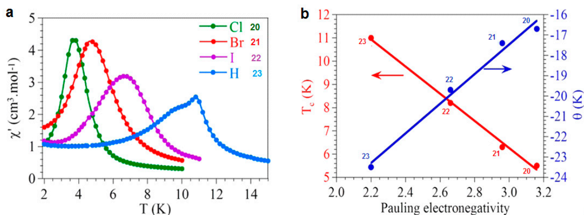
Figure 13. Magnetic properties of the [\text{NBu}_4][\text{MnCr}(\text{X}_2\text{An})_3] family, X = Cl ( 20 ), Br ( 21 ), I ( 22 ) and H ( 23 ): (a) Thermal variation of the in phase ( \chi_m' ) AC susceptibility at 1 Hz.; (b) Linear dependence of the ordering temperature ( T_c , left scale, red) and the Weiss temperature ( \theta , right scale, blue) with the electronegativity of the X group. Solid lines are the corresponding linear fits. Adapted with permission from Reference [125]. Copyright 2013 American Chemical Society.
