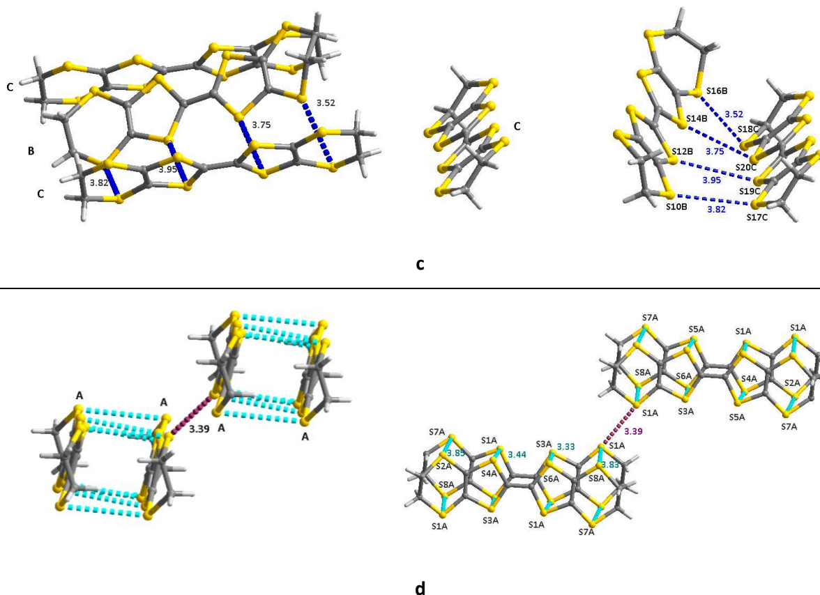
Figure 6.9. a) Unit cell showing the BEDT-TTF molecules. b-d) zoom pictures highlighting the interactions in the BEDT-TTF layer. Intra- and Inter-layer S...S contacts are highlighted. Face-to-face interactions are highlighted in A-A blue, B-B green. side-to-side interactions between B-C in dark blue, A-B in pink, A-A in violet, A-C in orange.
