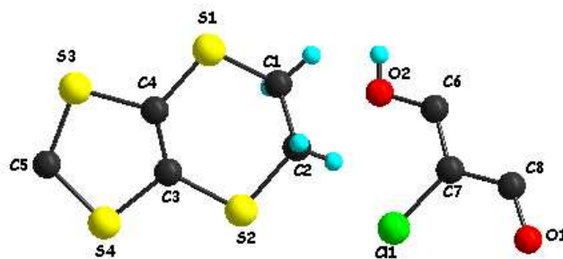
Figure 5.4. View of the independent half of molecules of donor and anion of the asymmetric unit in the structure of 2 together with the atom numbering scheme. H atoms are shown in cyan color.
