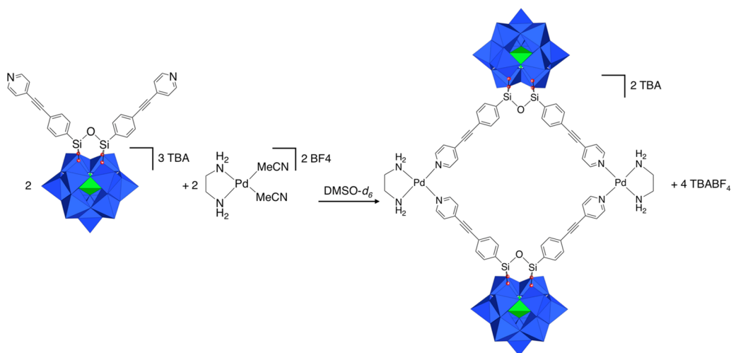
Figure 1. Metal-driven formation of the molecular square from the POM hybrid K_{Si}[pyr] .
