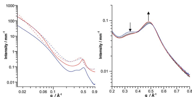
Fig. 10 (Left) SAXS pattern the POM.Co^{II} organogels: K_{Sn}[tpy].Co^{III} (plain blue), K_{Sn}[tpy].Co^{II} (plain red), D_{Sn}[tpy].Co^{III} (dotted blue) and D_{Sn}[tpy].Co^{II} (dotted red). (Right) Evolution of the SAXS pattern of K_{Sn}[tpy].Co^{III} under successive acquisitions; the bold blue and red lines correspond to the first and last scans respectively. The solvent and the capillary were subtracted to obtain these patterns.
