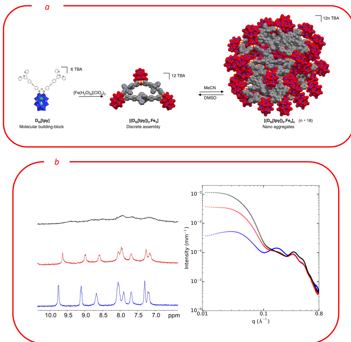
Figure 22 – (a) Schematic representation of the formation of the nanosized aggregates by hierarchical self-assembly of D_{5i}[tpy] upon complexation with Fe^{2+} . (b) ^1H NMR spectra and (left) and SAXS curves (right) of solutions of D_{5i}[tpy] (1 mM) in the presence of 1 equiv. of [Fe(H_2O)_6](ClO_4)_2 in DMSO- d_6 (blue), DMSO- d_6/CD_3CN (1/1) (red), and DMSO- d_6/CD_3CN (1/4) (black). G. Izzet et al.; J. Am. Chem. Soc., 2016, 138, 5093-5099.
