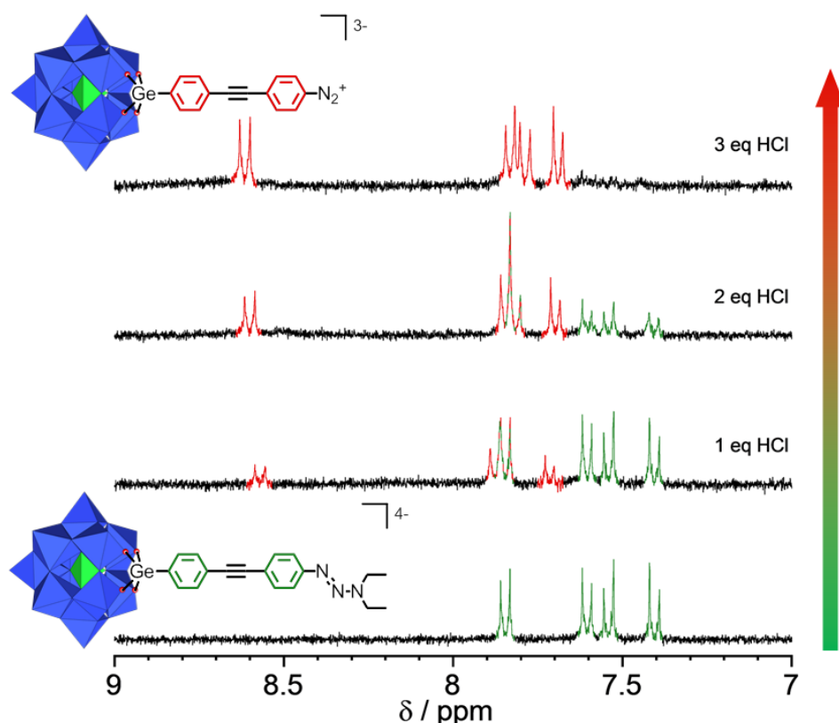
Figure 43 – ^1\text{H} NMR monitoring of \text{K}_{\text{Ge}}[\text{N}_2^+] formation from \text{K}_{\text{Ge}}[\text{N}_3\text{Et}_2] by addition of HCl in \text{CD}_3\text{CN} . C. Rinfray, thesis, Université Pierre et Marie Curie, 2014.
