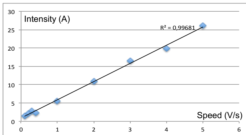
Figure 58 - CV of grafted POMs on ITO. (top) Keggin with Sn arm; (center) Keggin with Si arms; (bottom) Dawson with Si arms. 0.3 V.s -1 . (Graph) first reduction peak relative maximum intensity (A) evolution with speed (V/s)
