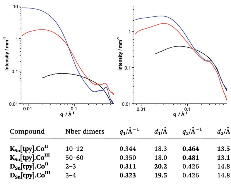
Figure 33 – Top: SAXS pattern of a 1 mmol solution of the molecular building-unit K_{Sn}[tpy] (left, black curve) and D_{Sn}[tpy] (right, black curve) and the resulting aggregates POM.Co^{II} (red curves) and POM.Co^{III} (blue curves) assemblies in CD_3CN . Bottom: data extracted from the SAXS curves of K_{Sn}[tpy].Co^{II} , K_{Sn}[tpy].Co^{III} , D_{Sn}[tpy].Co^{II} and D_{Sn}[tpy].Co^{III} in CD_3CN solution, d = 2\pi/q ; values in bold correspond to the main peak. M. S. Centallas et al.; Chem. Sci., 2020, 11, 11072-11080.
