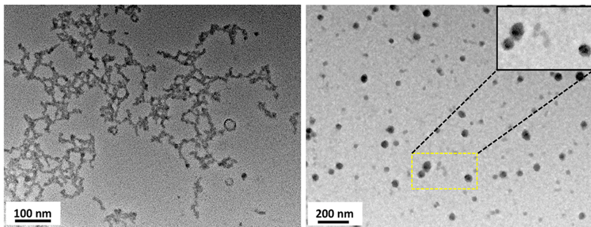
Figure 28 – TEM micrograph of the POM-Pd assemblies in DMSO/D 2 O 1:1 (left) and DMSO-d 6 /CD 3 CN 1:4 (right, magnification of three vesicles in the upper right corner) mixtures. R. Salles et al.; Inorg. Chem. , 2020, 59, 2458-2463.
