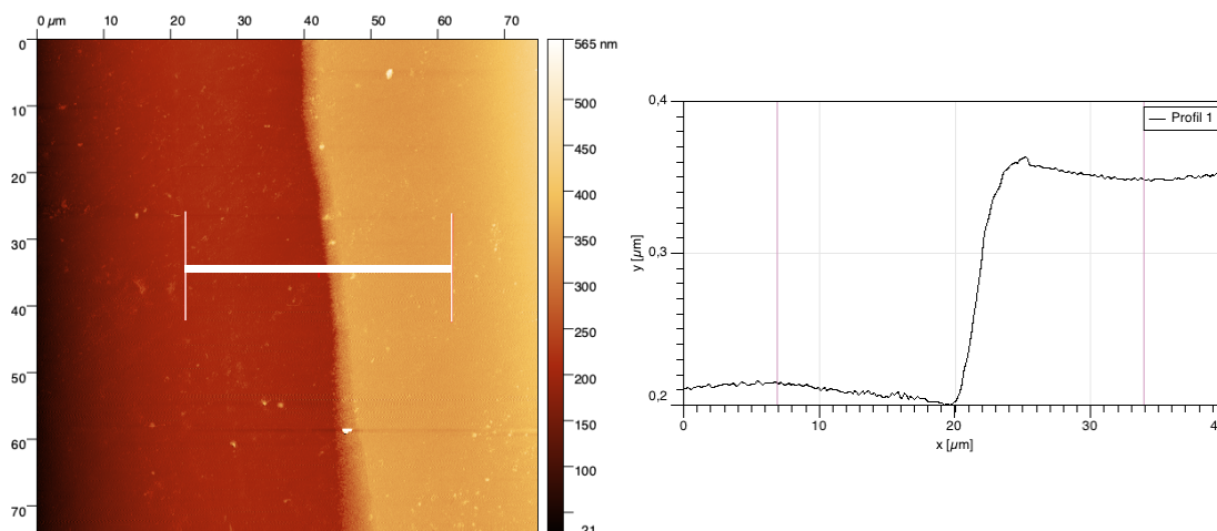
Figure 67 – (top) Measured height (in nm) of the two interfaces on 6 different POMs double grafted substrates. (bottom) AFM image and corresponding topographic profile of etched ITO substrate after D_{Si}[ArNH_2] double grafting, at the interface between glass (red, left) and ITO + POM (orange, right) areas.
