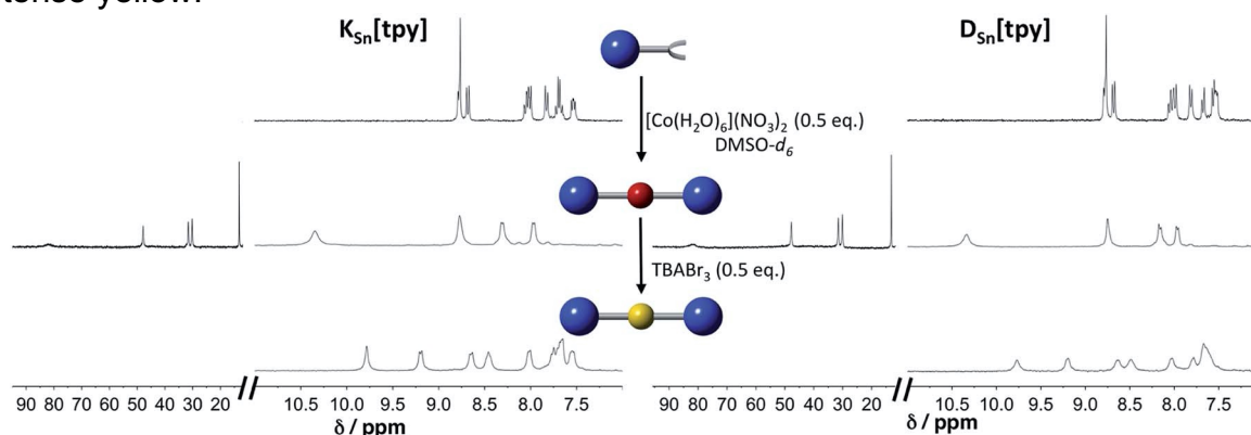
Figure 31 – 1 H NMR (300 MHz) in DMSO- d 6 solution containing K Sn [tpy] (2mM, top left) and D Sn [tpy] (top right) in the presence of 0.5 equiv. of [Co(H 2 O) 6 ](NO 3 ) 2 (middle); after oxidation of the Co(II) with 0.5 equiv. TBABr 3 (down). M. S. Centallas et al.; Chem. Sci., 2020, 11, 11072-11080.
