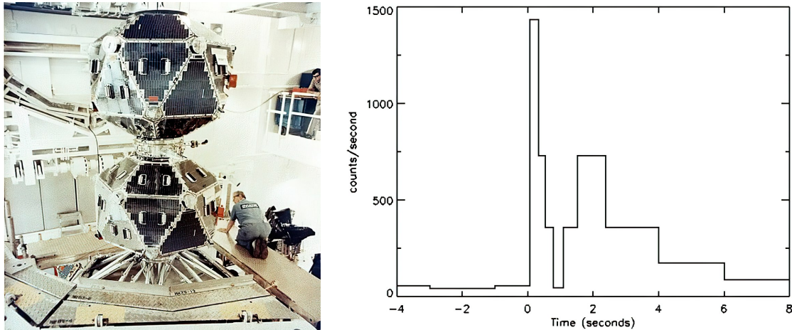
Figure 1.1: Left panel: Picture of the Vela-5A/B satellites in their cleanroom. (Credit: Los Alamos National Laboratory). Right panel: The light curve of the first gamma-ray burst detected on July 2, 1967 by the Vela 4A/B and the still operational Vela 3 satellites (Credit: Bonnell 1995).
