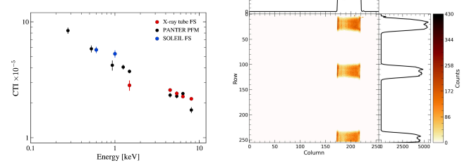
Fig. 5: Charge transfer inefficiency ( 1 - \text{CTE} ) computed from 3 runs per energy and comparison with data obtained with the X-ray source in the lab (comparable pixel flux but full illumination).
