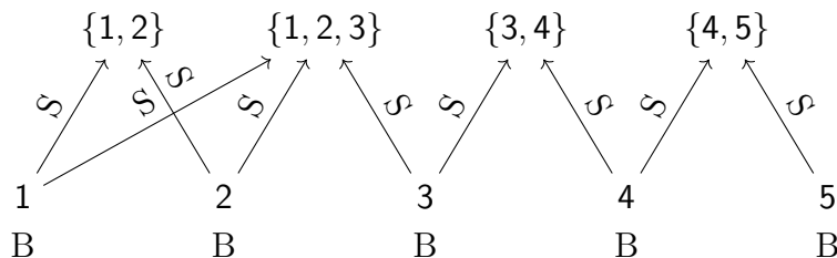
Figure 5.2: The built ABox for the example instance of SET COVER.
