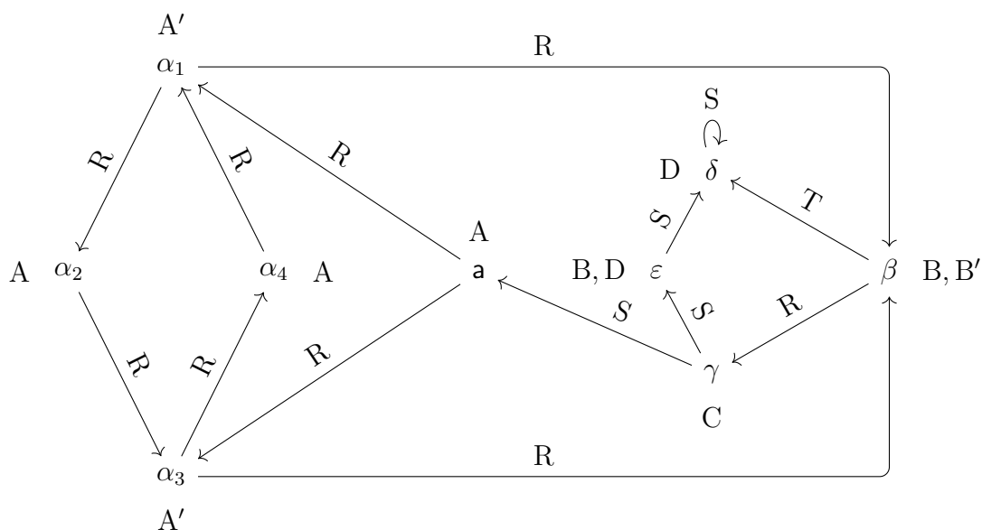
Figure 3.6: Model \mathcal{I}_e of \mathcal{K}_e
