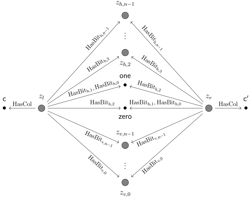
Figure 3.15: The subquery q^{\mathcal{H},(c,c'),2} to check an horizontal tiling condition.
