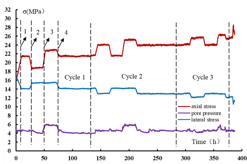
Figure V .7: Stress evolution with time in lateral decompression test
