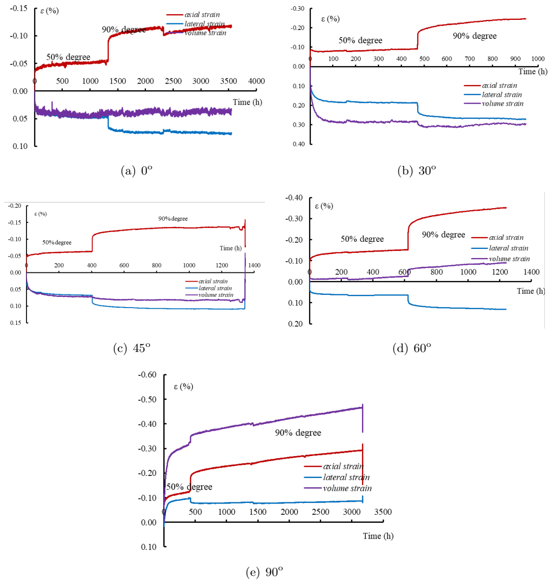
Figure III .5: Strain-time curve evolution for axial extension tests
