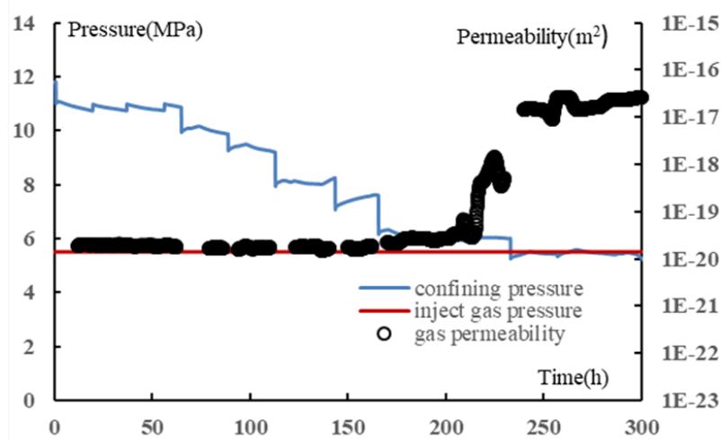
Figure IV .27: Evolution of gas permeability, confining pressure and gas pressure with time in unloading process for fractured sample C17
