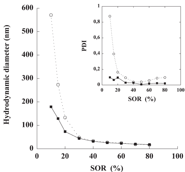
Fig. 2 Nano-emulsions formulated with non-iodinated oil (open circles) and iodinated oil (filled squares). Surfactant = Cremophor ELP®, oil = (native or iodinated) Labrafil M 1944 CS®. Hydrodynamic diameters are plotted against the surfactant oil weight ratio (SOR). Inset : The corresponding polydispersity indices are plotted vs. SOR.
