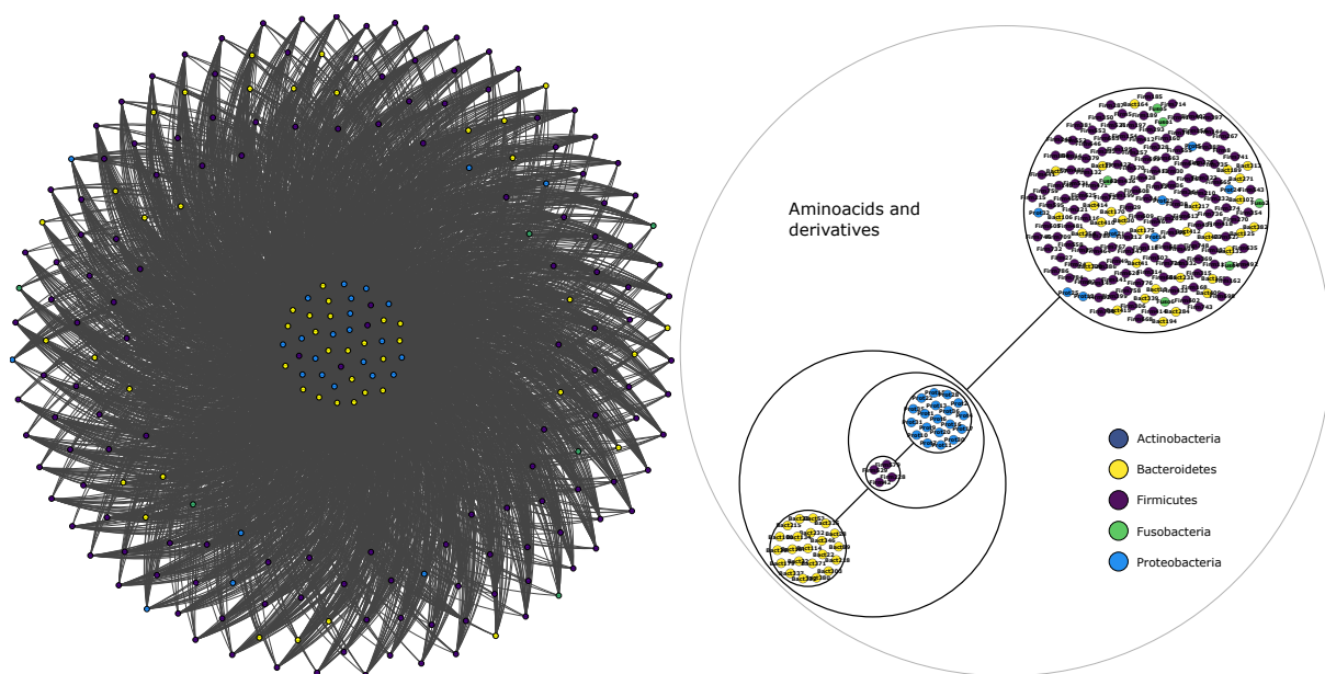
Figure 5.3 – At the left, the solution graph shows the minimal communities for the amino acids and derivatives targets. Nodes represent the organism in the minimal community. Edges are drawn between nodes in the same minimal communities. Right power graph compressing the information of the previous graph.
