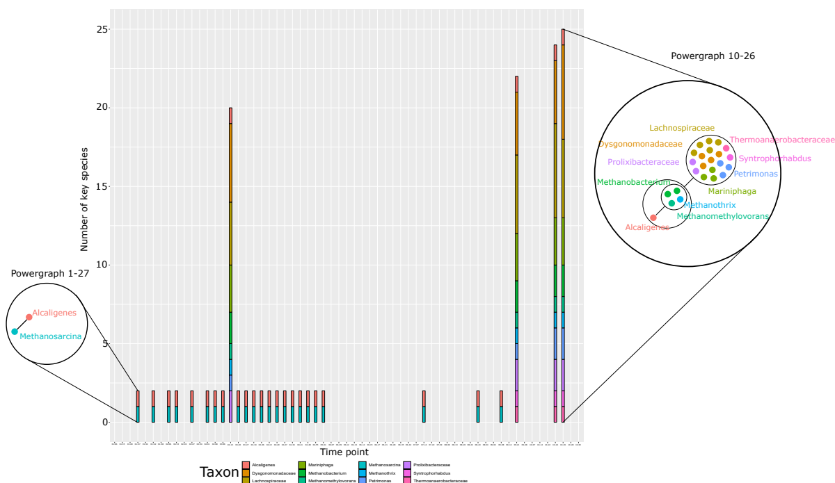
Figure 5.5 – Power graph showing the key species producing the targets for each time point, according to the sequenced OTUs.
