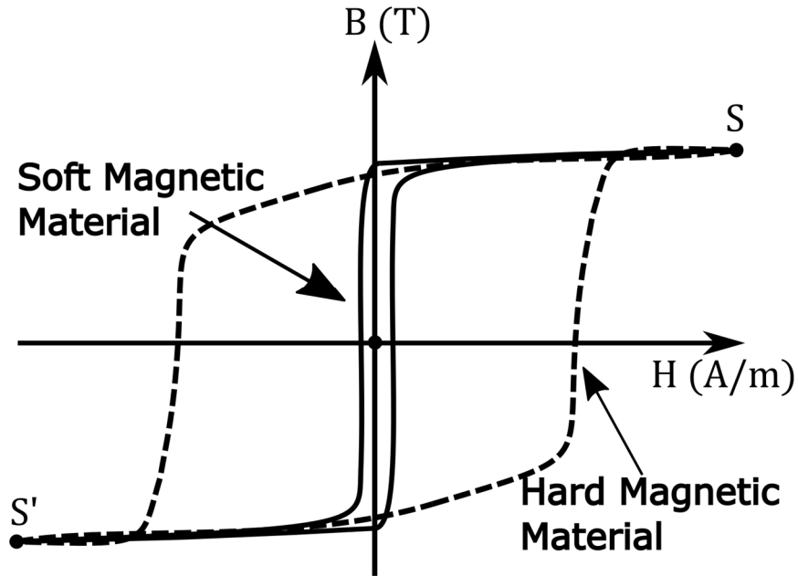
Fig. II-3 Illustrative hysteresis loops for soft and hard magnetic materials.
