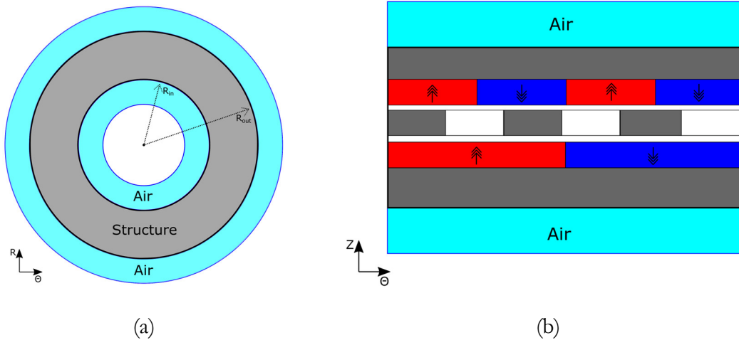
Fig. II-21 2D projections of an axial field MG with the air envelope on the (a) (R, \theta) plane and (b) (\theta, Z) plane.
