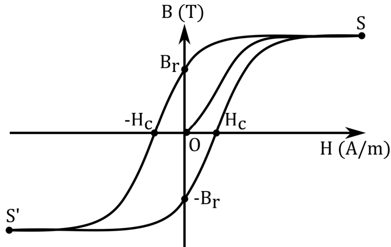
Fig. II-2 A typical B-H plot or hysteresis loop.
