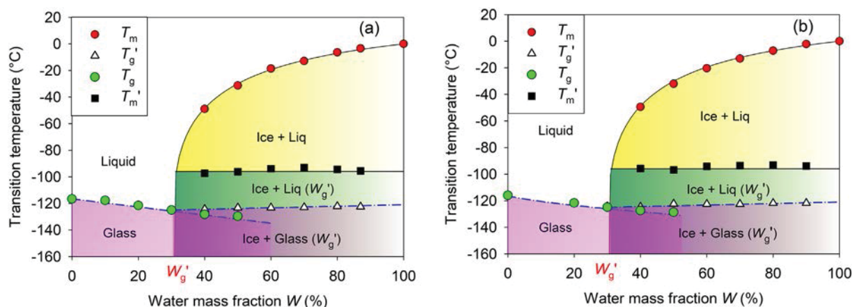
Fig. 5. Phase diagram of aqueous solutions of Ethaline DES mixtures as a function of the water mass fraction W for two molar compositions of Ethaline (a) Ethylene Glycol/Choline Chloride in a 2:1 mol ratio and (b) Ethylene Glycol/Choline Chloride in a 3:1 mol ratio.
