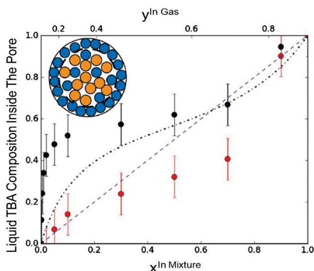
Figure IV-13: Final TBA composition of the liquid inside the MCM-41 pores after capillary condensation versus the original composition x^{In\ Mixture} (black circles). The red circles show the deduced composition of the liquid in the core of the pore within the frame of a core-shell model (with only TBA at the surface). As a guide to the eye: the dashed line indicates the composition of the original liquid mixture, and the dash-dotted line indicates the composition of the gas phase. Inset: Scaled schematic representation of the completely filled MCM pore in the frame of a core-shell model with blue to indicate tert-butanol molecules and orange for toluene ones.
