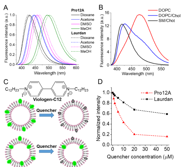
Figure 2. Spectroscopy experiments in solvents and lipid vesicles. (A) Normalized fluorescence spectra of Pro12A and Laurdan in solvents of different polarities. (B) Fluorescence spectra of Pro12A in LUVs of different compositions. Probe concentration was systematically 2 \mu\text{M} . Total lipid concentration for all vesicles was 1 \text{ mM} . (C) Chemical structure of Viologen-C12 and scheme of surface quenching by Viologen-C12 of the probes located at the outer bilayer leaflet (upper panel) and both leaflets (lower panel). (D) Fluorescence quenching of Pro12A and Laurdan in DOPC LUVs with increasing concentrations of Viologen-C12. The intensity was recorded at the maximum of probe emission: 476 \text{ nm} (Pro12A) and 493 \text{ nm} (Laurdan). Probe and lipid concentrations were 1 and 500 \mu\text{M} , respectively. Twenty millimolar phosphate buffer (pH 7.4) was used for all LUVs. \lambda_{\text{ex}} = 360 \text{ nm} in all cases.
