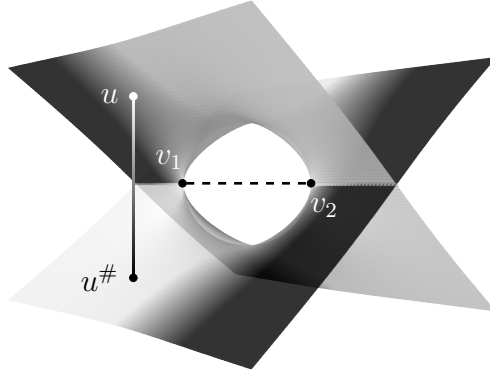
FIGURE 4.4.2 – A graphical representation of \Omega_\delta^{\bullet[v_1, v_2]} locally around the branching given by v_1, v_2 \in \Omega_\delta^\circ . The vertices u, u^\# \in \Omega_\delta^\bullet are two different vertices belonging to the same fiber.
