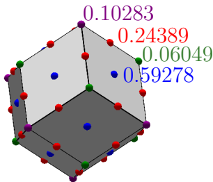
Figure 4.7: The scaled Voronoi cell and the optimal coefficients for F(2, 8) . Supporting points \alpha in the same Weyl group orbit and their additive inverse \hat{\alpha} have the same coefficients, denoted by red, blue, green and purple dots.
