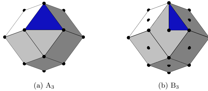
Figure 4.6: The rhombic dodecahedron is the Voronoi cell of the lattice of coroots for A_3 and B_3 .
