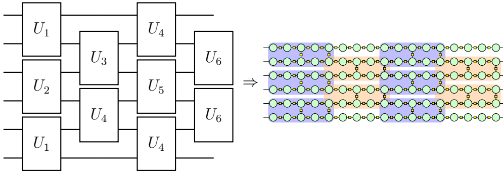
Figure 2.6: Composing multiple gates in an MBQC computation. The nodes which are not colored in the pattern are supposed to have phase 0, or for efficiency reason they can also be replaced with wires. Other nodes have phases corresponding to the gates.
