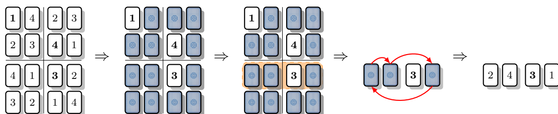
Figure 7.1: Illustration of ZK with a small sudoku (in bold). On the first image, Alice has a solution to the sudoku. Then, she hides this solution by flipping the cards (second image). Bob challenges Alice to reveal one line (in orange, third picture). Alice shuffles this line (fourth picture) and shows that it contains all numbers exactly once (last picture). Bob learns no information beside the fact that this line contains all numbers exactly once. Then, the process restarts from scratch: Bob can challenge other lines/columns/blocks until he is convinced that Alice really knows a solution to the sudoku.
