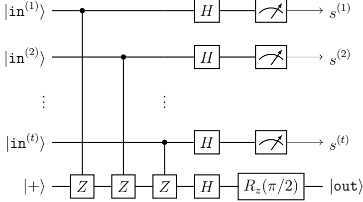
Figure 4.5: The XOR gadget circuit \text{Gad}_{\oplus} (run on server side). Note that the rightmost Hadamard and rotation on the last wire is only used to bring a |+\theta\rangle back into a BB84 state. When using other protocols that actually expect |+\theta\rangle states (the first step of the \mathbb{Z}_4^{\pi} -QFactory protocol undoes this operation) we can remove them. We see that this circuit has been simplified since the our original publication (thanks ZX-calculus).
