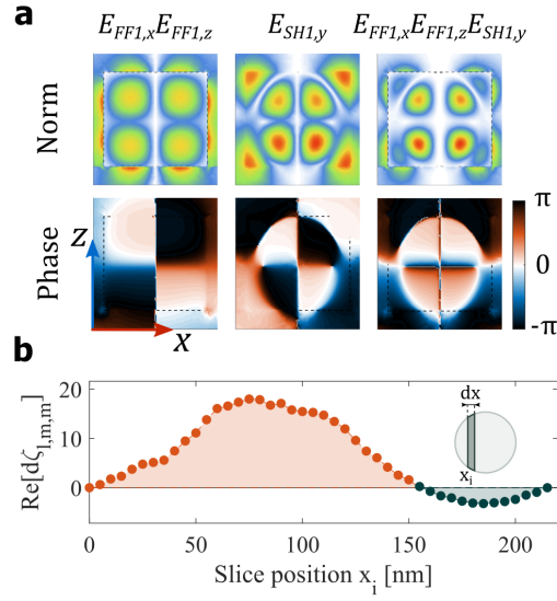
Figure 3.8: Nonlinear overlap analysis between modes FF1 and SH1. (a) Main components of the modes: norm (top) and phase (bottom). From left to right: product of x and z components of \tilde{\mathbf{E}}_{FF1} ; y component of \tilde{\mathbf{E}}_{SH1} ; main component of the nonlinear product \tilde{\mathbf{E}}_{SH1} \cdot [\chi^{(2)} : \tilde{\mathbf{E}}_{FF1} \otimes \tilde{\mathbf{E}}_{FF1}] . (b) Discretized contribution to the overlap integral \zeta_{lmn} along finite slices in the xy plane, centered at x_i with thickness dx = 5 nm. Only the real part is reported.
