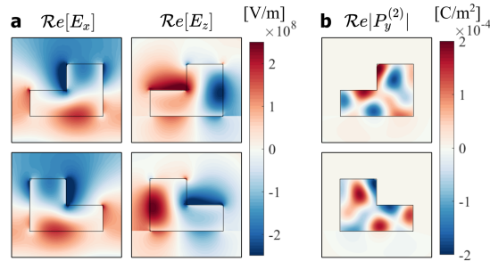
Figure 5.14: (a) x - (left) and z - (right) electric near-field components at \lambda_{FF} = 1550 nm for the same nanochair upon an in-plane rotation of 180^\circ . An input pump intensity I_0 = 1 GW/cm 2 is considered. (b) y -component of the second order polarization vector at \lambda_{SH} = 775 nm for the two cases.
