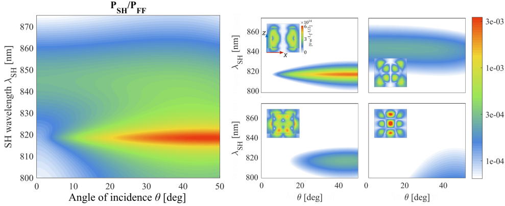
Figure 3.7: Ratio between SH ( P_{SH} = W_{ext}^{(2)} ) and FF ( P_{FF} = S_0 \pi r^2 ) power impinging on the AlGaAs-on-AlOx cylinder of Fig. 3.3. \theta is the angle of incidence between the plane-wave k -vector and the cylinder axis ( z ). S_0 is set at 1 \text{ GW/cm}^2 . The total reconstruction on the left is decomposed in its four main contribution on the right. Insets: near-field distributions |\tilde{E}_m| of the corresponding QNMs in the xz plane (the color bar is the same for the four plots).
