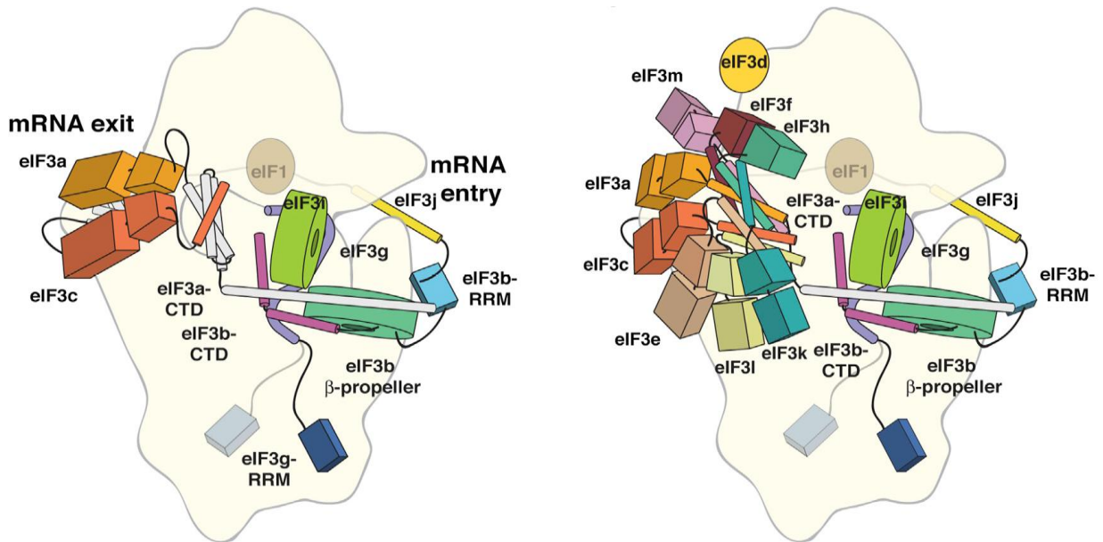
Figure 2.1-2 Placement and interactions of eIF3 components on 40S
