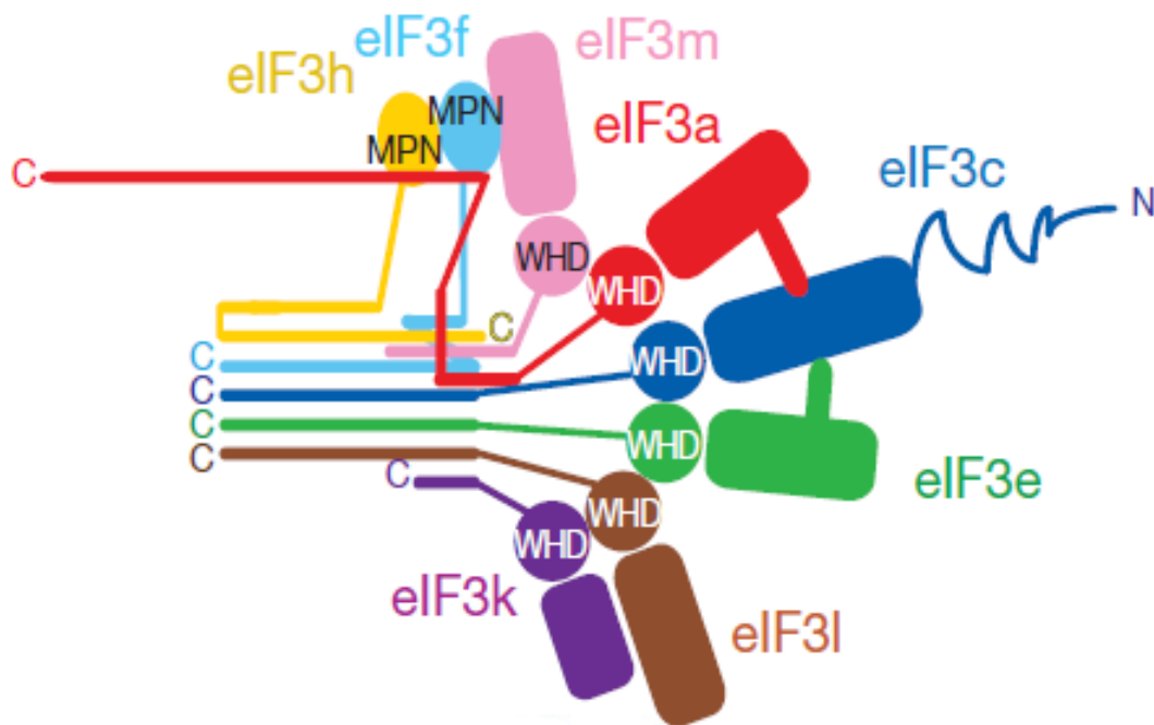
Figure 2.1-3 Two-dimensional representation of the eIF3 octamer core
