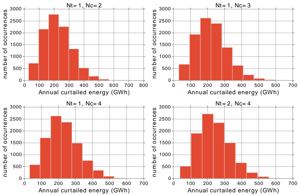
Figure 6-1: Empirical probability distributions of L_S^{cur}(X) obtained with 10 000 Monte Carlo simulations.
