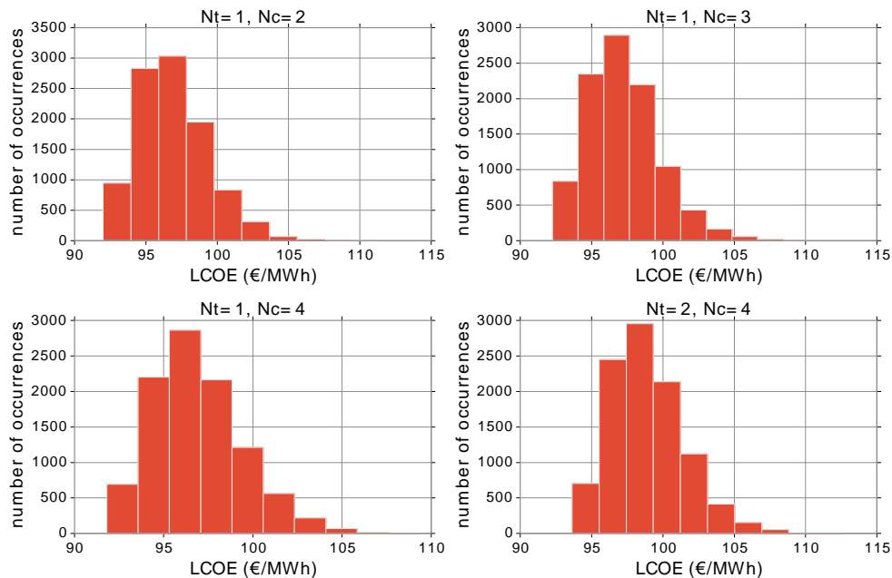
Figure 6-3: Empirical probability distributions the LCOE obtained with 10 000 Monte Carlo simulations.
