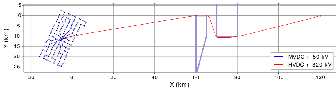
Figure 5-18: The optimal layout for N_T = 1 with the architecture (d)
