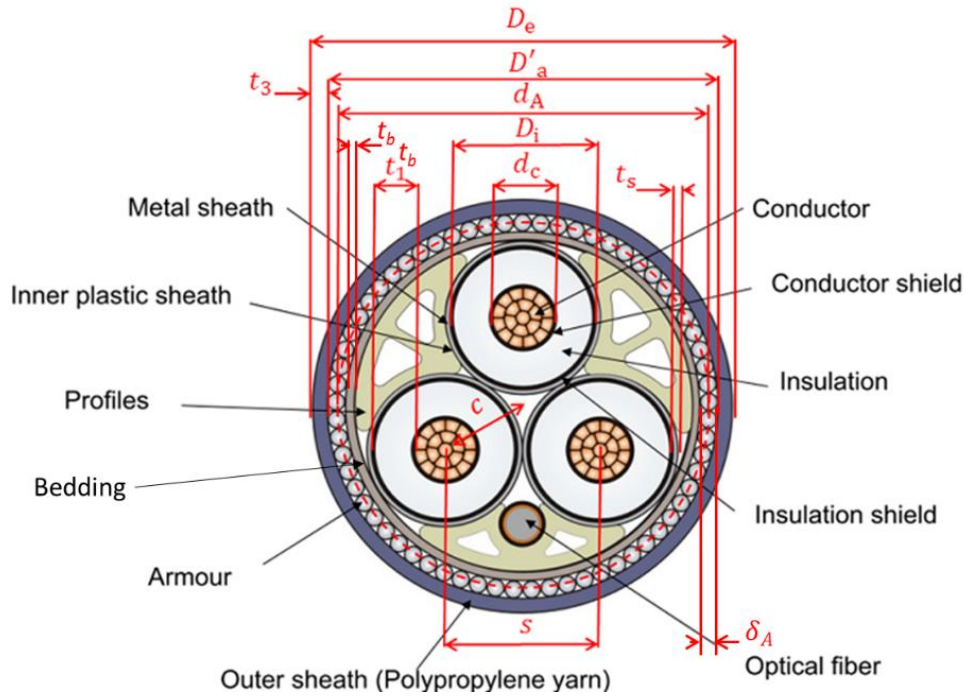
Figure A-1: Submarine AC cable layers and geometrical parameters definition
