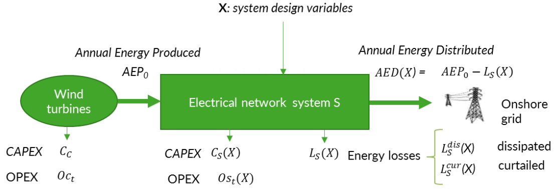
Figure 1-19: Schematic representation of the electrical network system connecting an offshore wind farm to the shore and definition of elementary indexes.
