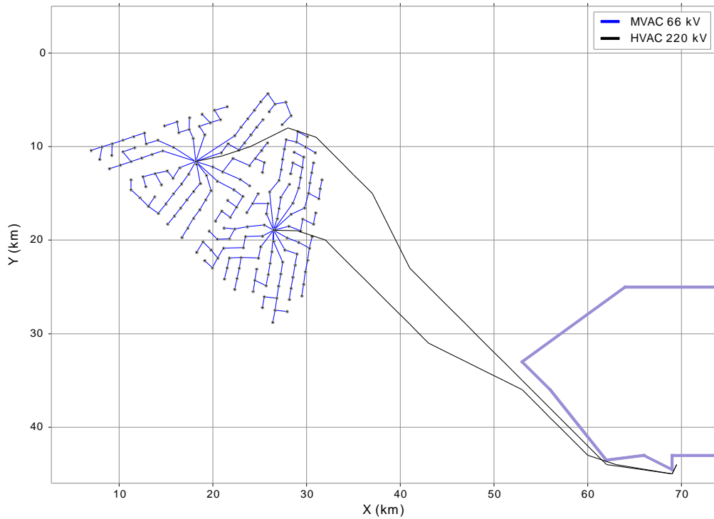
Figure 5-6: Electrical network layout for Borssele III and IV with (P2) solved with EW_MLCMS
