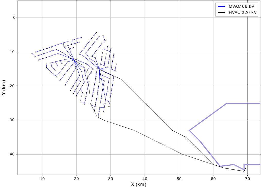
Figure 5-8: Electrical network layout for Borselee III and IV with Ecofys collection cables routing
