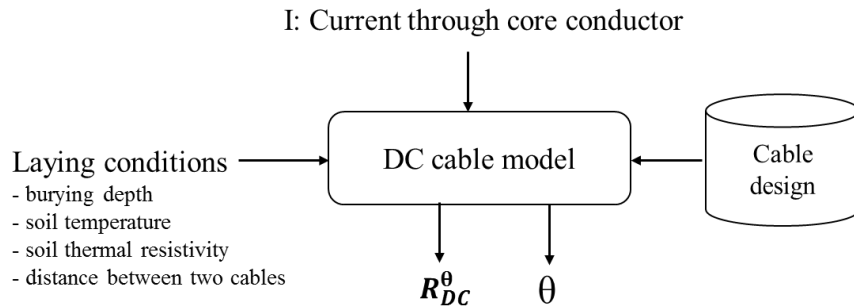
Figure 2-9: Synoptic diagram of the DC cable model
