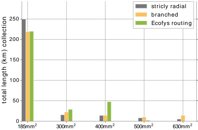
Figure 5-9: Obtained lengths of collection cables
