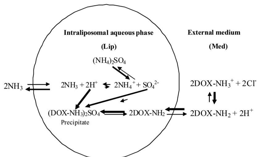
Figure 7. Doxorubicin remote loading by a transmembrane ammonium ion gradient, the bold arrows ( \rightleftharpoons ) represent the processes which occur during drug loading, while simple arrows ( \rightarrow ) represent the processes which occur during drug release.
