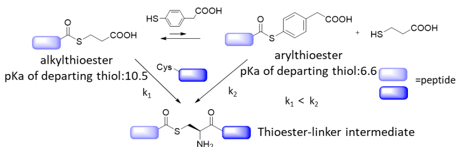
Scheme 2.13 | The catalytic mechanism of the NCL process in the presence of acidic thiols.
