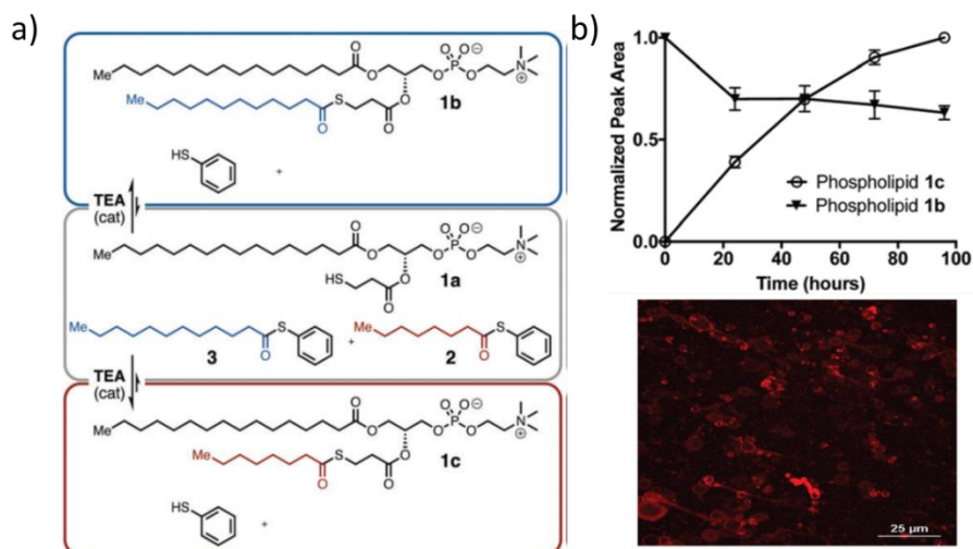
Figure 1.29 | Illustration of the formation of synthetic phospholipids using the thiol–thioester exchange reaction. Figure is reproduced and adapted from ref. 84 .
