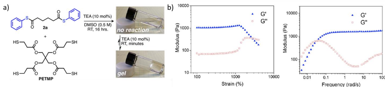
Figure 1.28 | a) Formation of a cross-linked polythioester organogel via transthioesterification; b) Oscillatory rheology of the polythioester hydrogel. Figure is reproduced and adapted from ref. 83 .
