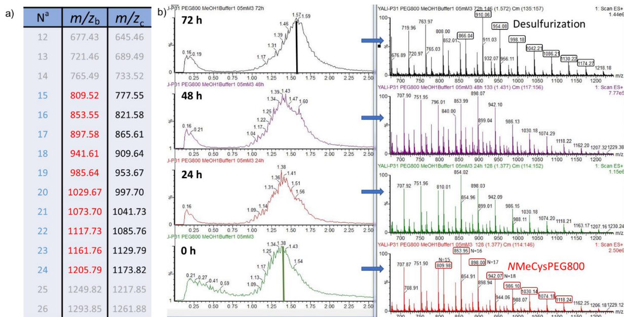
Figure 3.4 | a) Theoretical m/z_b for N MeCys-PEG800 and corresponding theoretical m/z_c for its desulfurization products as a function of ethylene oxide units ( N^a ). b) Mass chromatograms of a stock solution of N MeCys-PEG800 at a concentration of 0.5 mM for different stock time (from bottom to top, t = 0, 24, 48, and 72 h) and the corresponding mass spectra. The stock solution was kept in a 1/1 (v/v) mixture of methanol and milli-Q water at pH 5 containing 150 mM TCEP and 300 mM sodium ascorbate.
