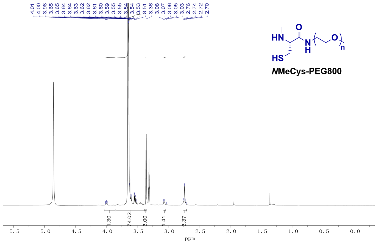
Figure A7 | ^1\text{H-NMR} spectrum of NMeCys-PEG800.
