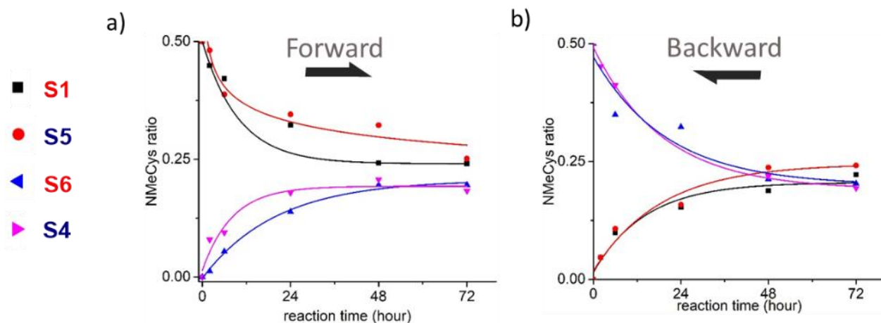
Figure 2.10 | Kinetic curves of the four constituents ( S1 , S4 , S5 , S6 ) of the library in acetonitrile (200 mM DTT) for the a) forward and b) backward direction. NMeCys ratio: [S1_{\text{reaction}}]/[S1_{\text{initial}}] , [S5_{\text{reaction}}]/[S1_{\text{initial}}] , [S4_{\text{reaction}}]/[S1_{\text{initial}}] and [S6_{\text{reaction}}]/[S1_{\text{initial}}] .
