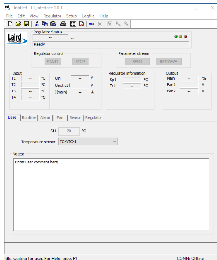
Figure A3.1: The LT-Interface (Laird Technologies) for manipulating in real time the input and output parameters of the TC-XX-PR-59 reversible controller.
