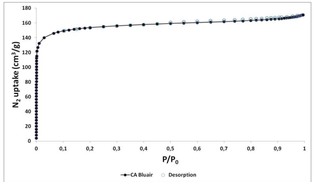
Figure A.45 : Adsorption/désorption de N 2 des CA.
