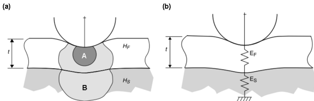
Figure 2.16: (a) Plastic zone in thin-film systems (of thickness = t ) on hard substrates (A) and soft substrates (B). (b) Elastic response of the film/substrate system represented by two springs connected in series. [185]
