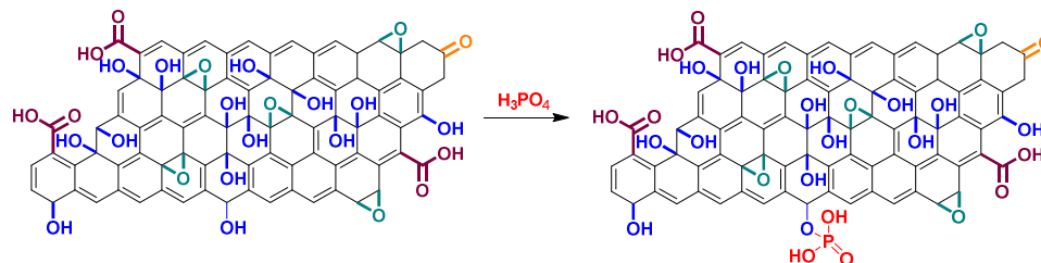
Scheme 1.4 Phosphorylation of GO. 67 (The reaction has been drawn only on one functional group for clarity reasons. Side reactions were not considered).
