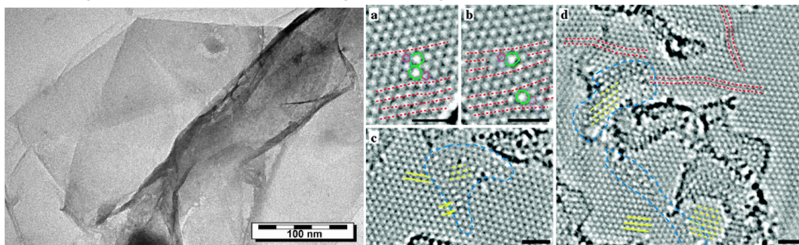
Figure 1.10 Left: TEM image of GO. 63 Right: HRTEM of reduced GO ("(a, b) Dislocation dipole observed at two different times (b) 2 minutes after a) in the TEM. Each dislocation core consists of a pentagon-heptagon pair. The separation between the dislocation cores has increased, indicating that there is a significant amount of strain present. (c, d) Defect cluster, indicated by blue dashed lines. Yellow dashed lines indicate the regions with hexagonal lattice rotated to the dominant orientation (yellow solid lines for comparison). Red dashed lines indicate again distortions in the hexagonal lattice. Yellow arrows in (c) indicate strongly elongated carbon polygons. All scale bars are 1 nm"). Adapted from reference 101.
