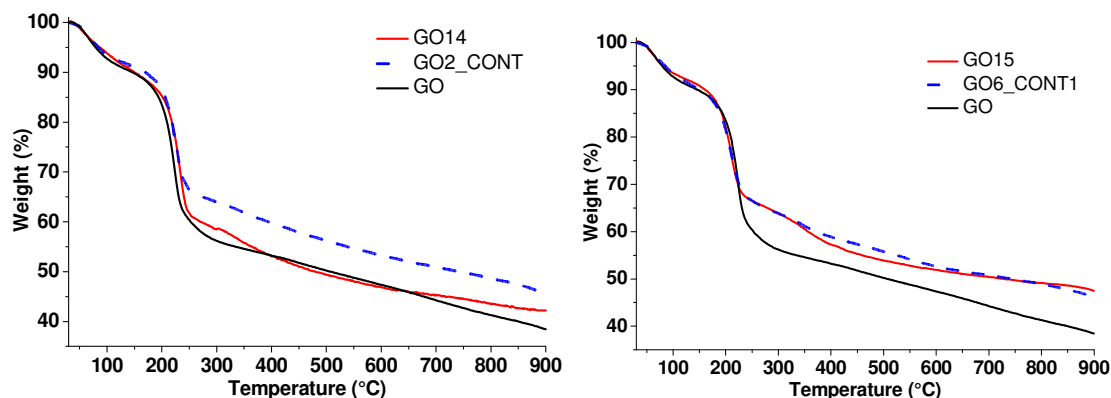
Figure 3.6 TGA curves of GO, GO14, GO15, GO2_CONT and GO6_CONT1.
