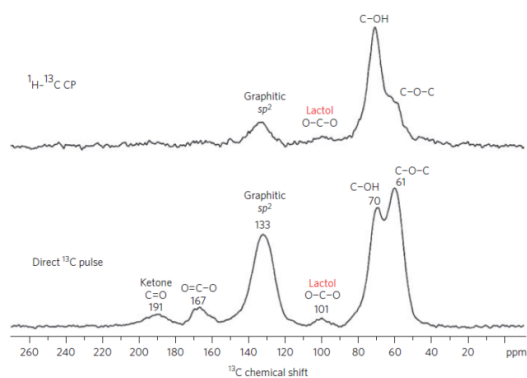
Figure 1.12 Top: 1 H- 13 C CP spectrum; Bottom: direct 13 C pulse spectrum of GO. Adapted from reference 64.
