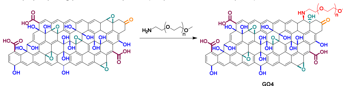
Scheme 2.4 Opening of epoxide GO4 (the reaction has been drawn only on one functional group for sake of clarity).
