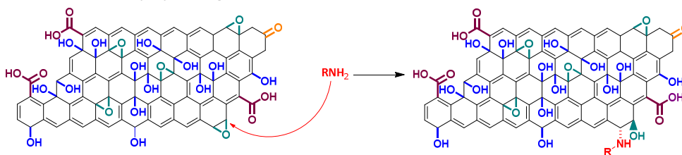
Scheme 1.9 Opening of epoxide ring on GO. (The reaction has been drawn only on one functional group for clarity reasons).
